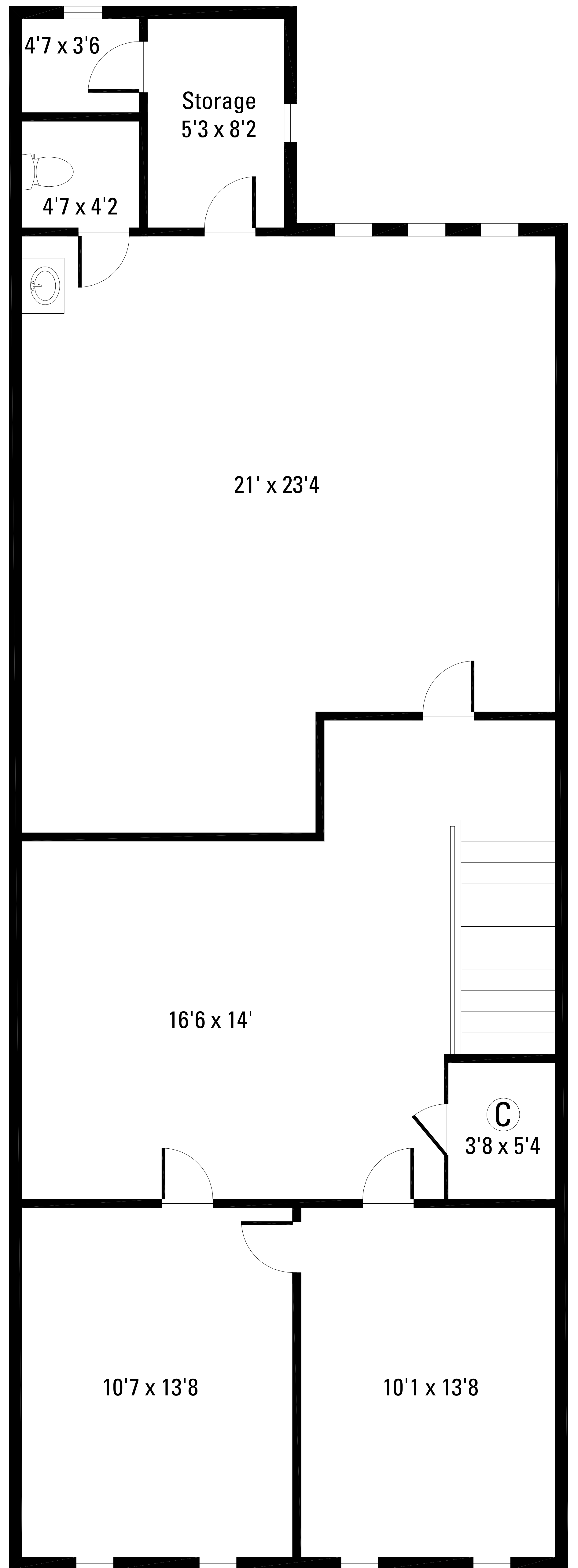
SECOND FLOOR
