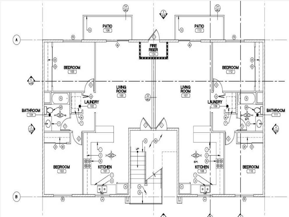
floor plan seco adobe
