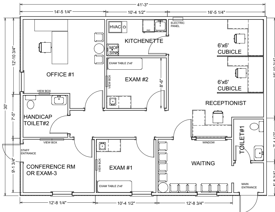
EXISTING FLOOR PLAN AS MEDICAL USE
