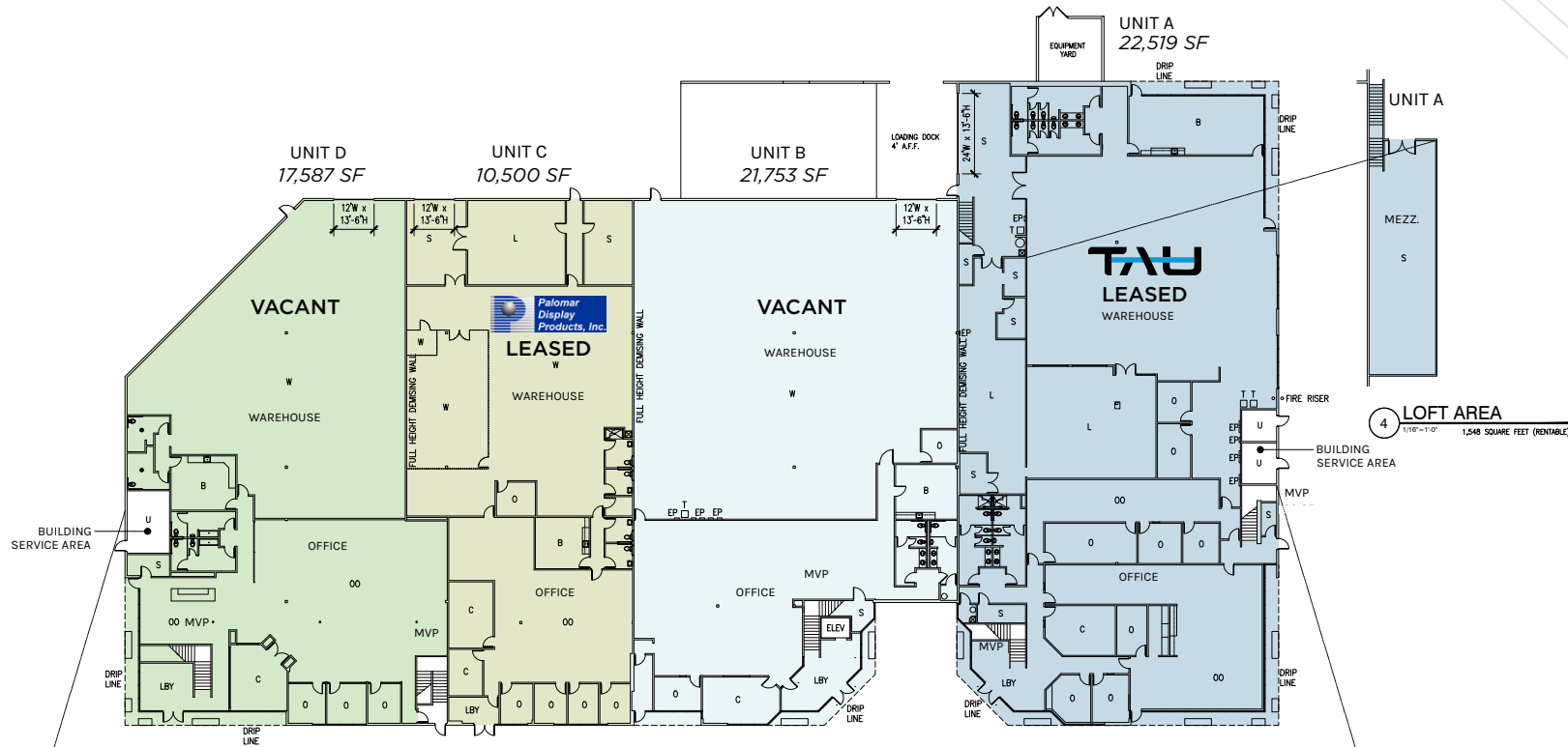
1 FIRST FLOOR PLAN 1/16" = 1'-0"
