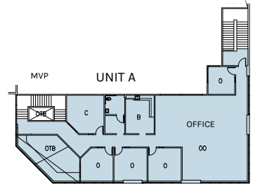
3 SECOND FLOOR PLAN 1/16" = 1'-0"
