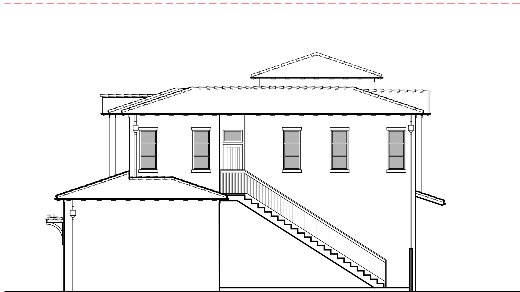
REAR ELEVATION
