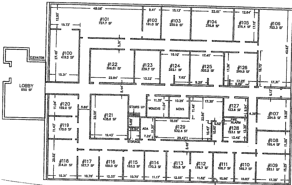
FLOOR 1
