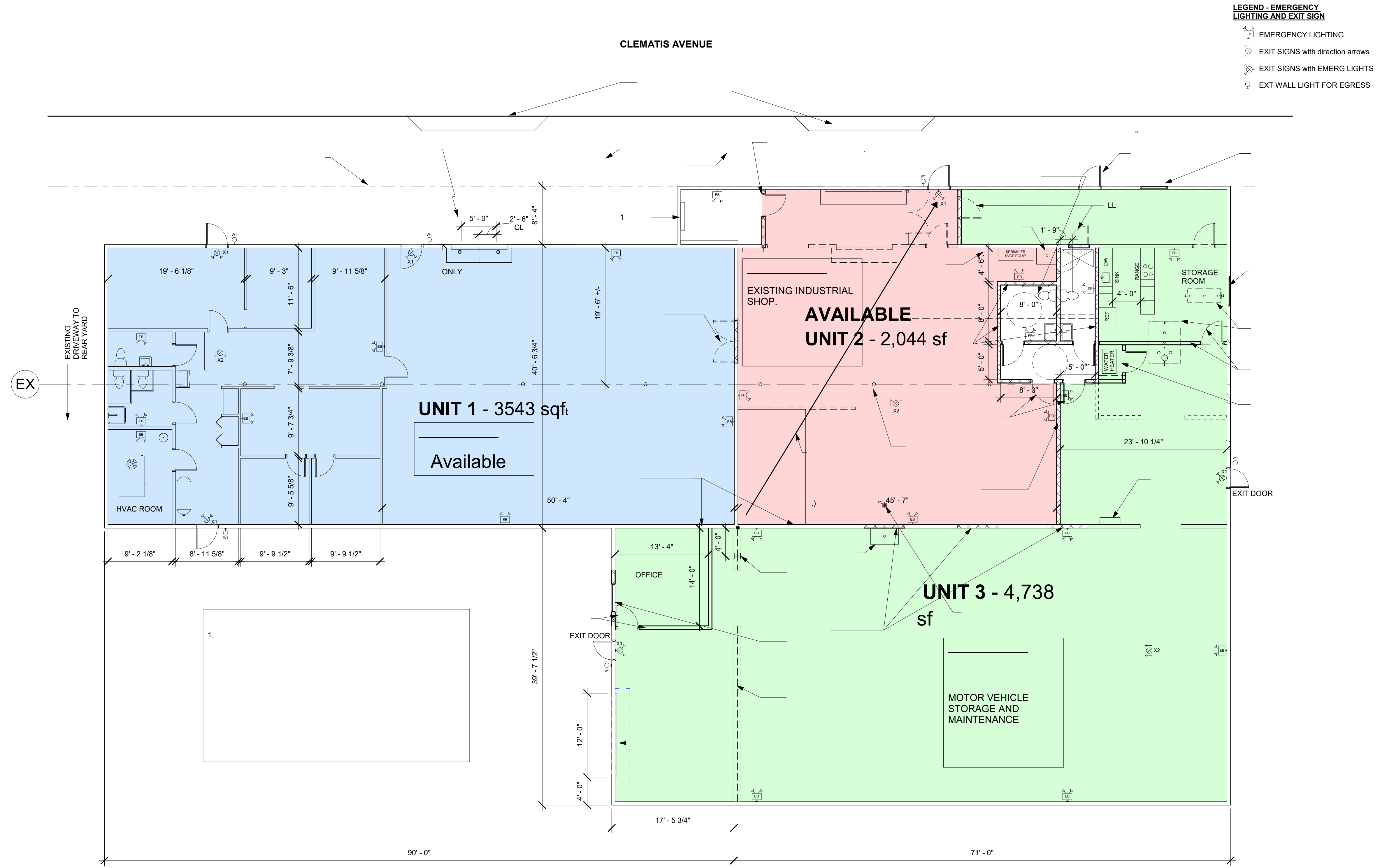
1 Floor Plan - Unit Demising Plan 1/8" = 1'-0"
