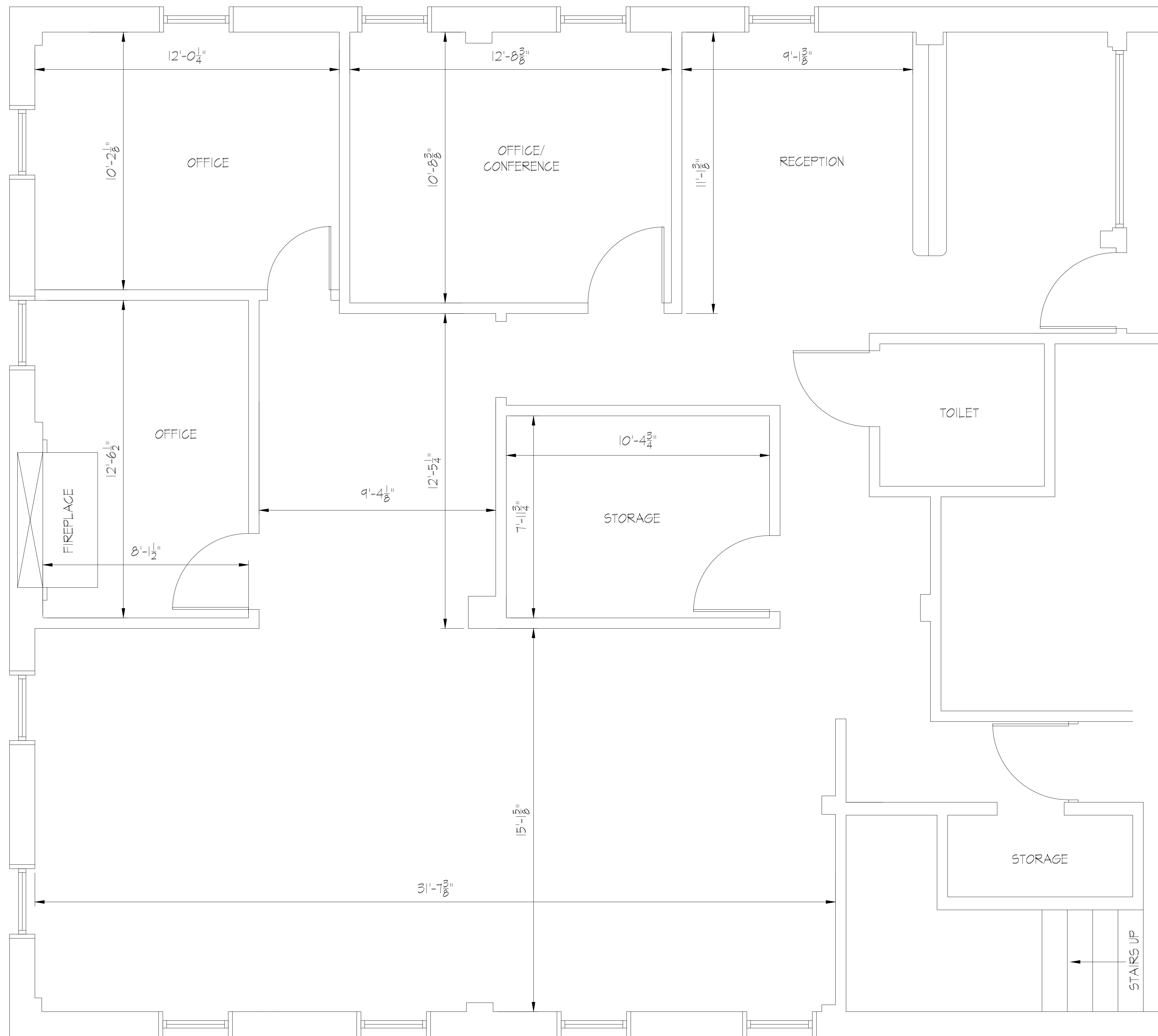
1 FLOOR PLAN 1/2" = 1'-0"
