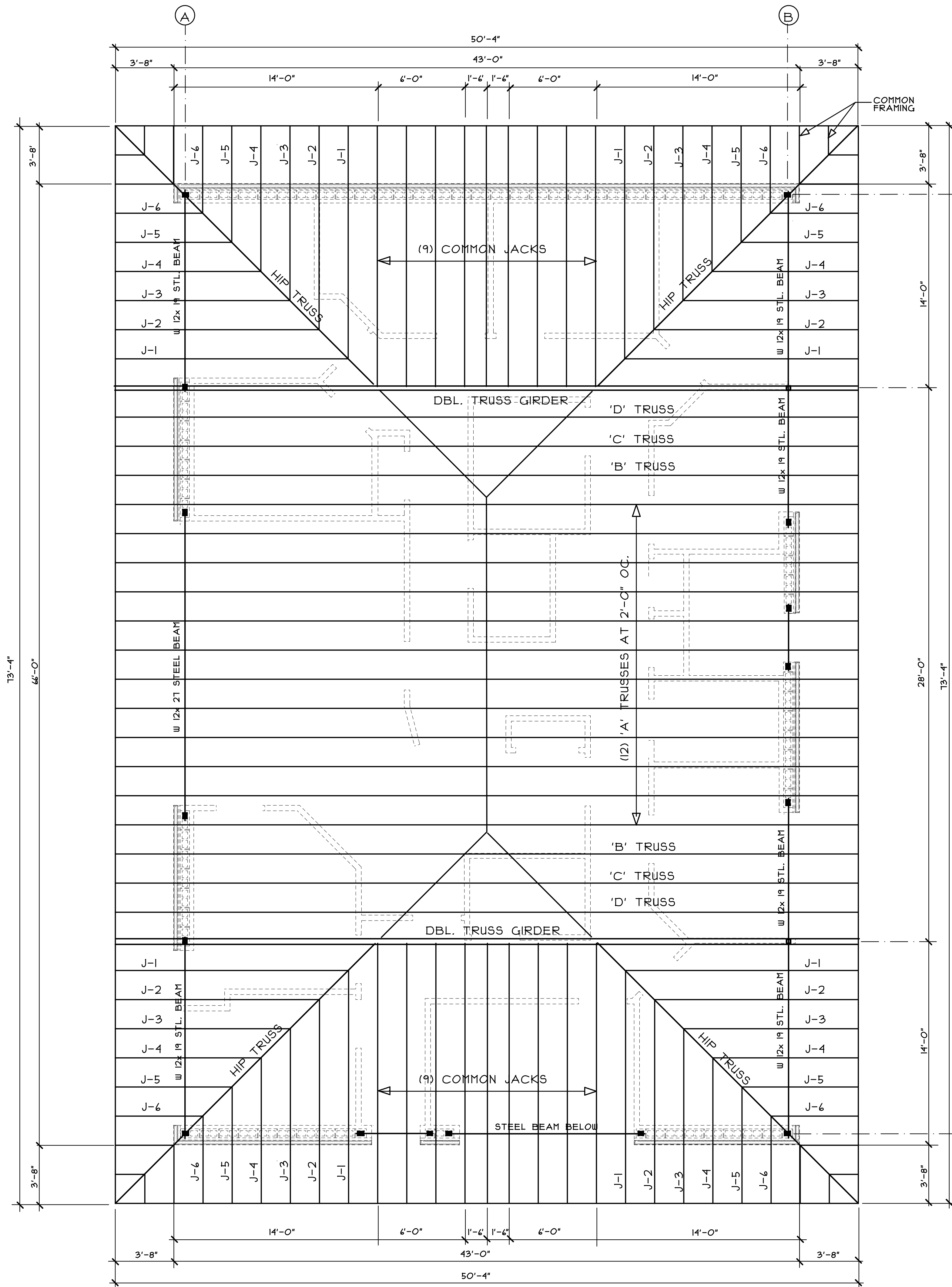
ROOF TRUSS FRAMING PLAN
