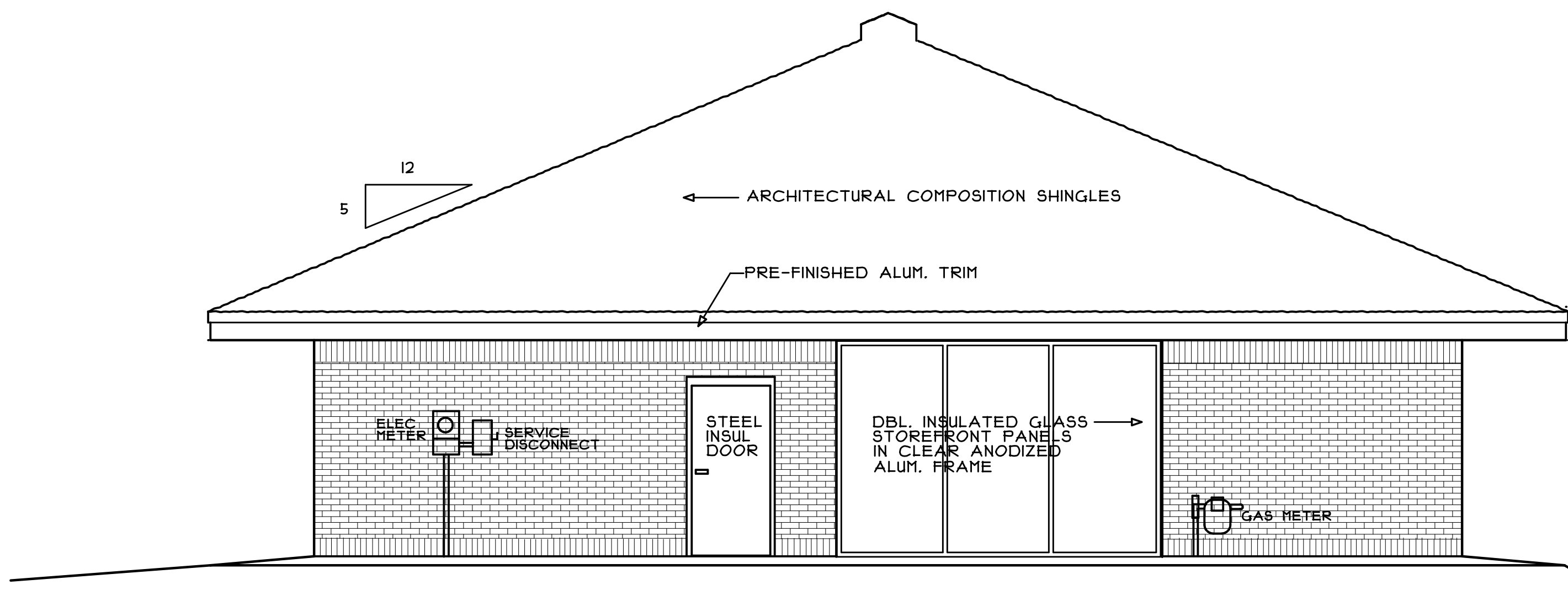
NORTH ELEVATION
