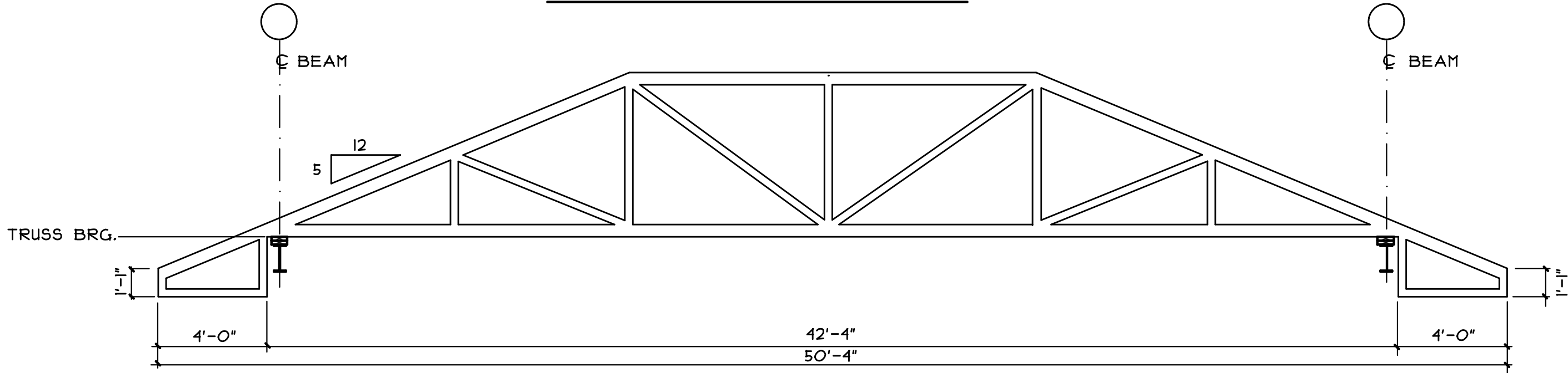
DBL. TRUSS GIRDER
