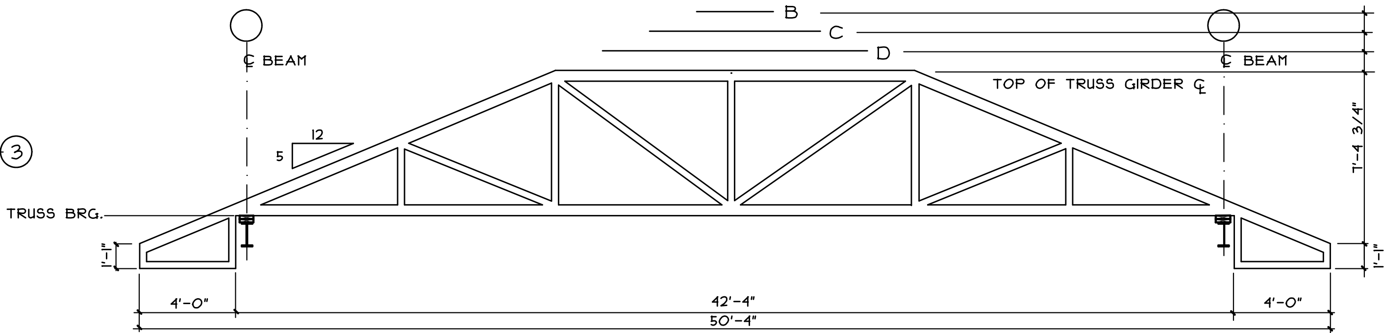
STEP DOWN TRUSSES - B, C, AND D
