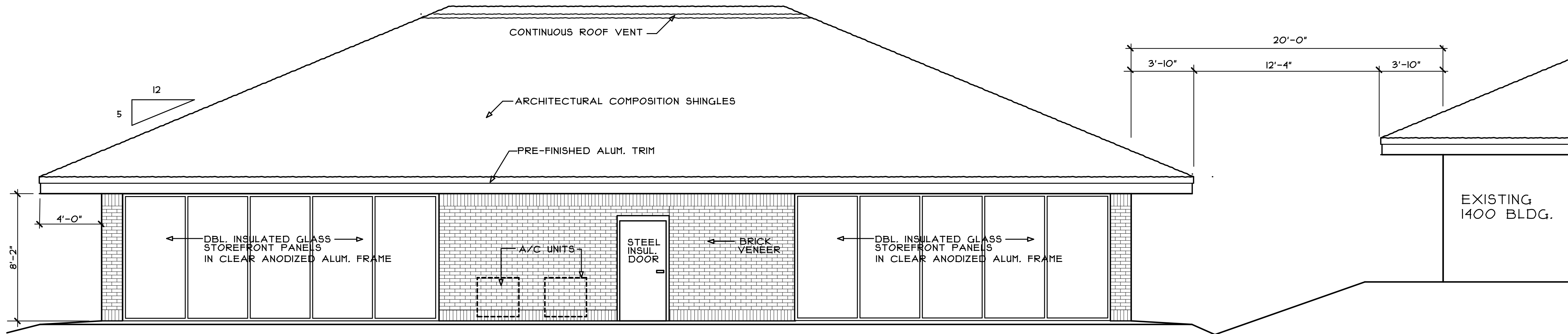
WEST ELEVATION (EXPRESSWAY SIDE)
