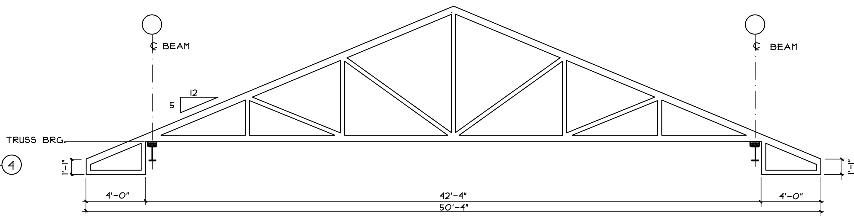
STANDARD TRUSS TYPE 'A'
