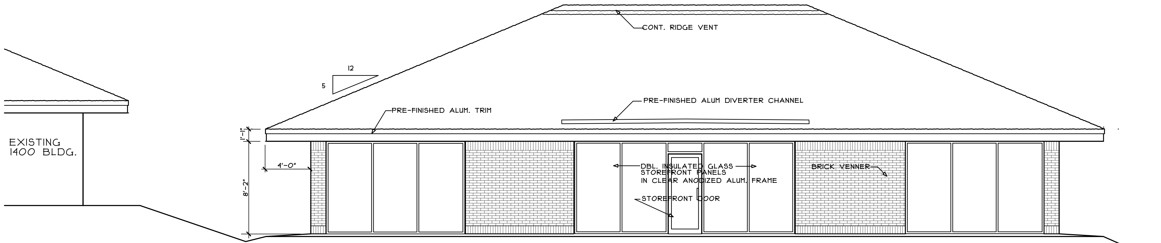
EAST ELEVATION (FRONT)
