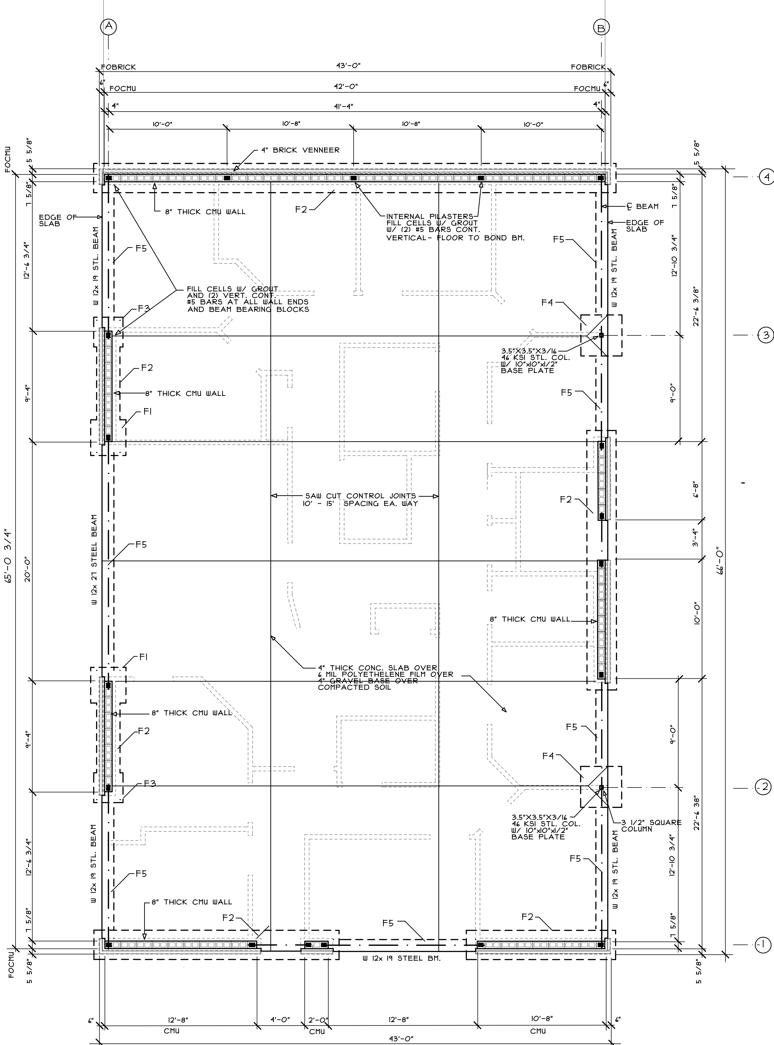
FOUNDATION PLAN SCALE: 1/4" = 1'-0"
