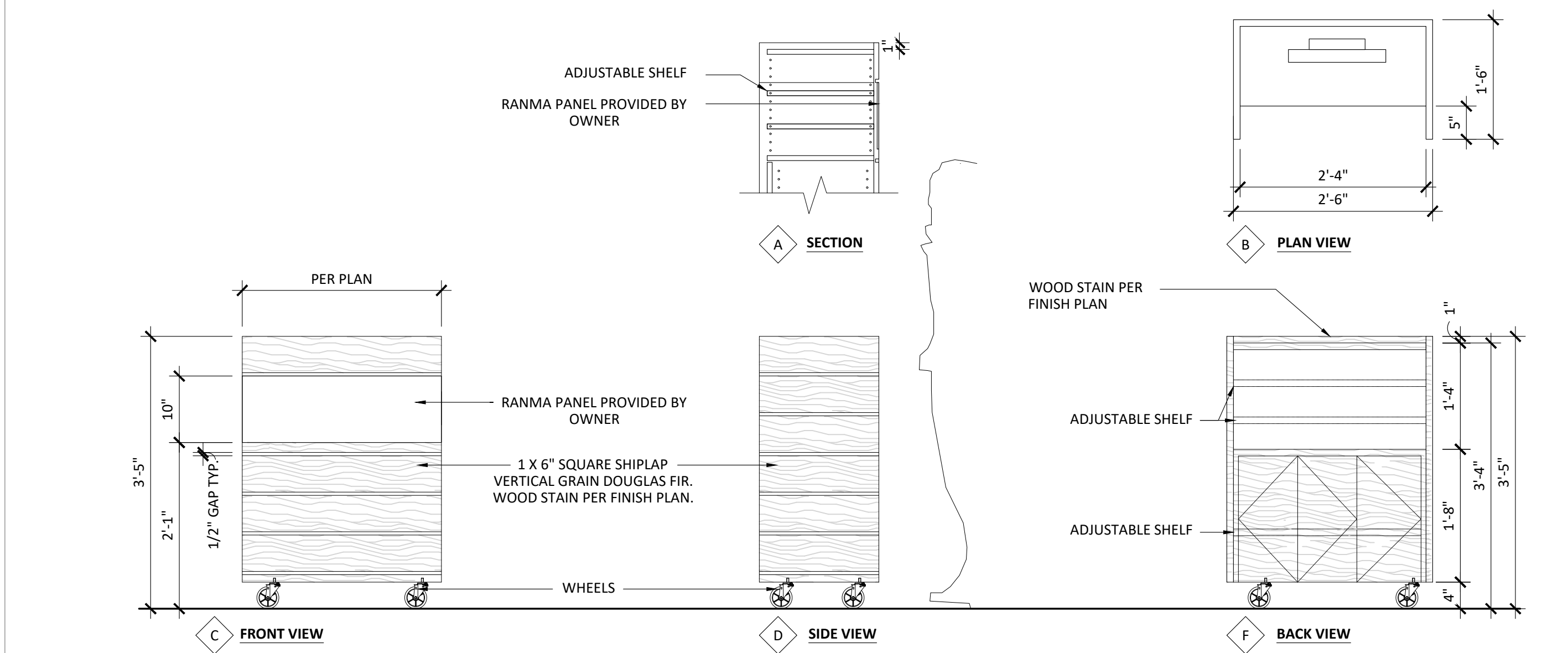
5 HOSTESS STAND DETAIL SCALE: 3/4" = 1'-0"
