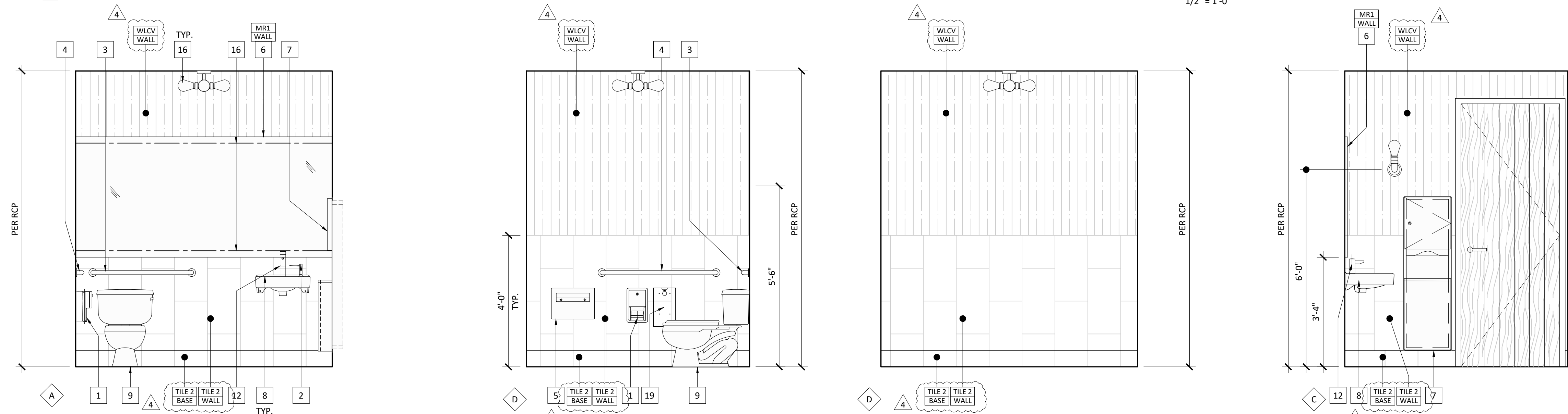
3 #108 WOMEN'S RESTROOM ELEVATIONS
