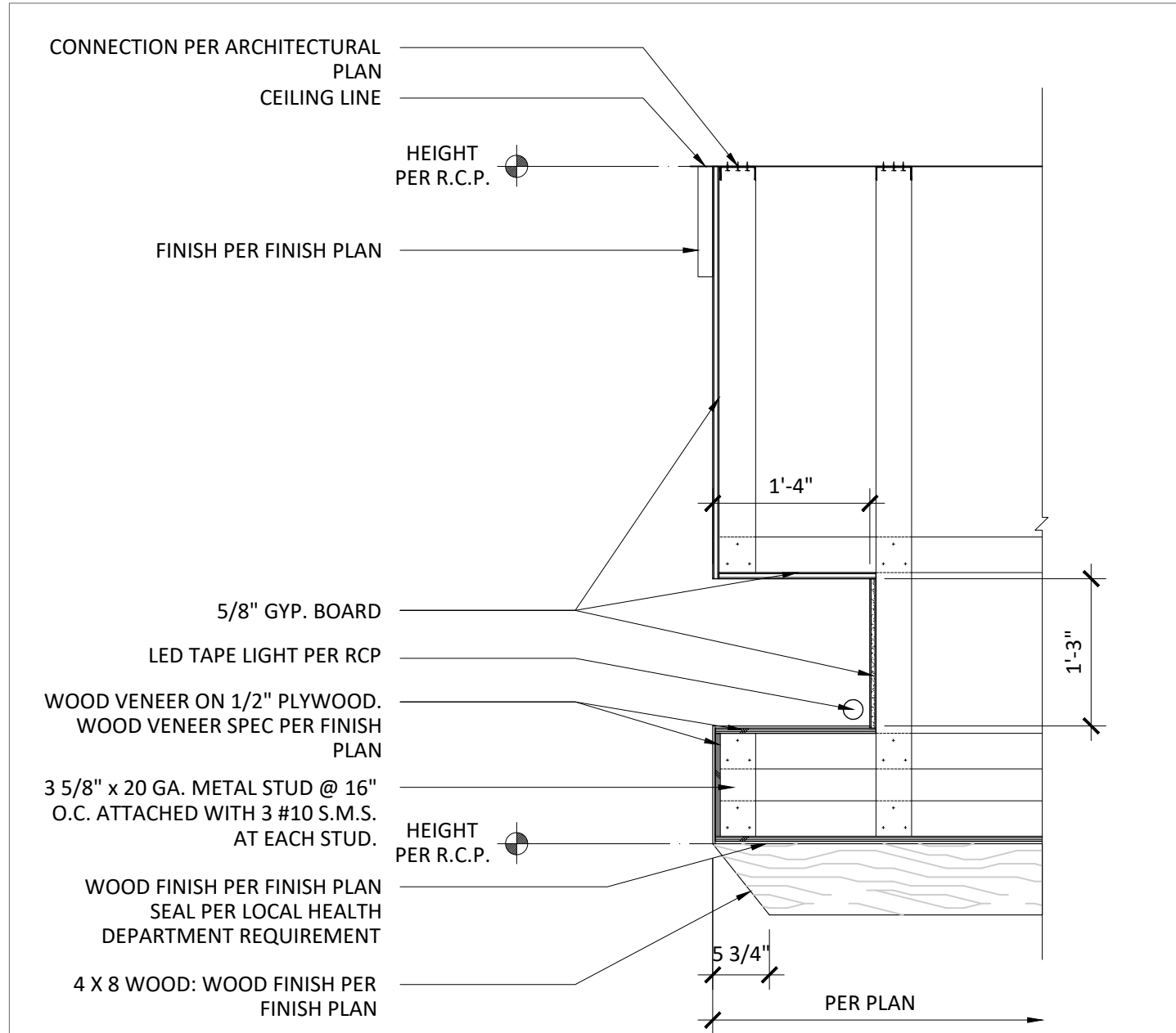
1 SOFFIT DETAIL @ ROBATA SCALE: 3/4" = 1'-0"
