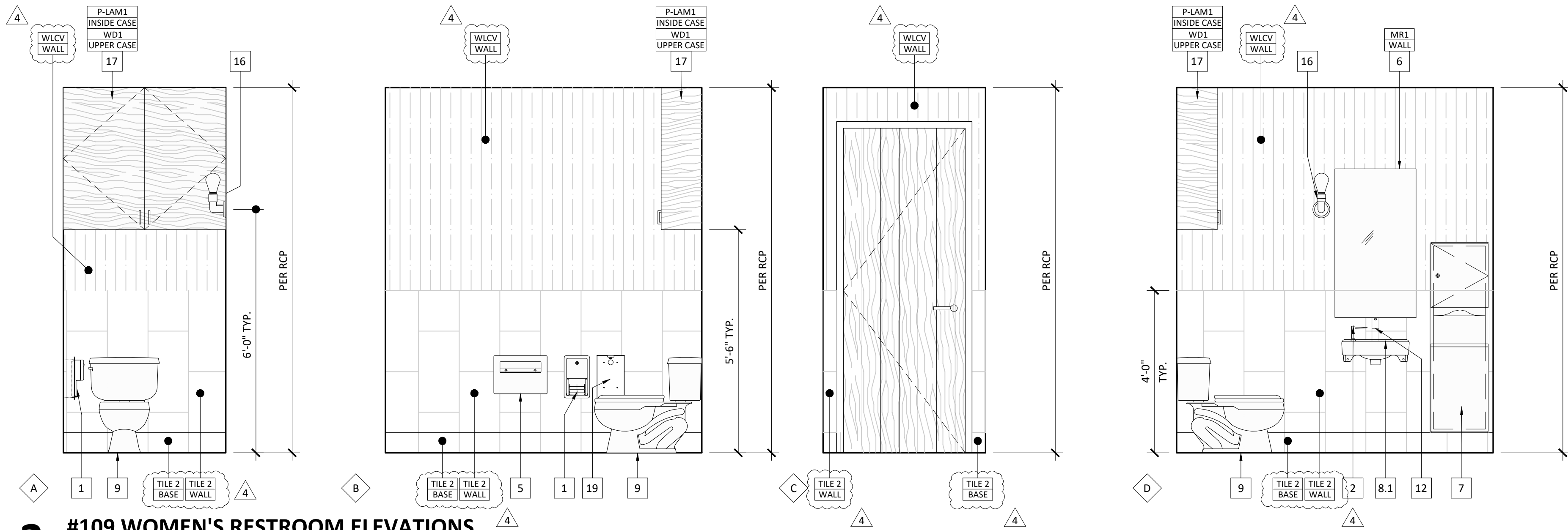
2 #109 WOMEN'S RESTROOM ELEVATIONS
