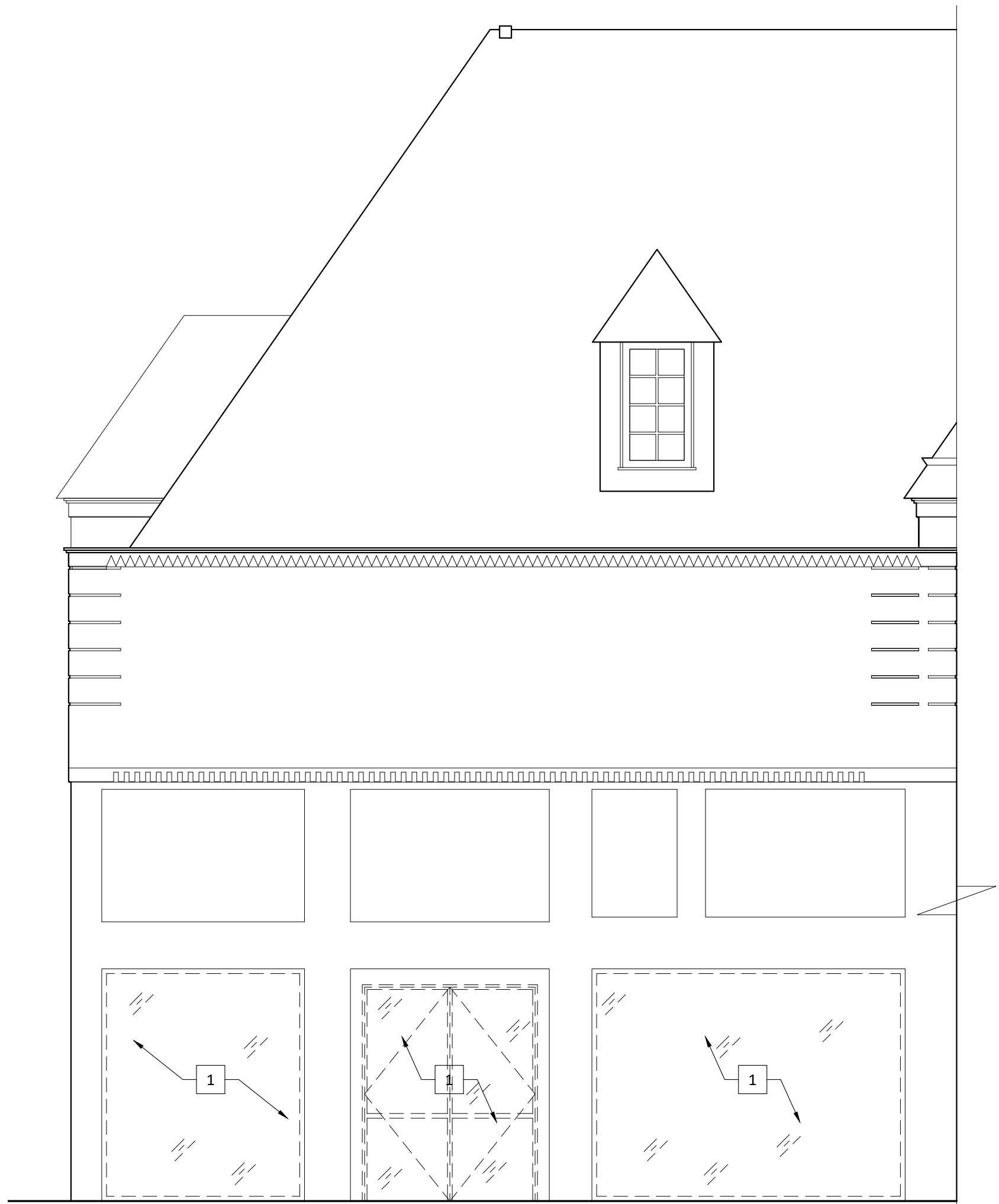
1 DEMOLITION SOUTH ELEVATION
