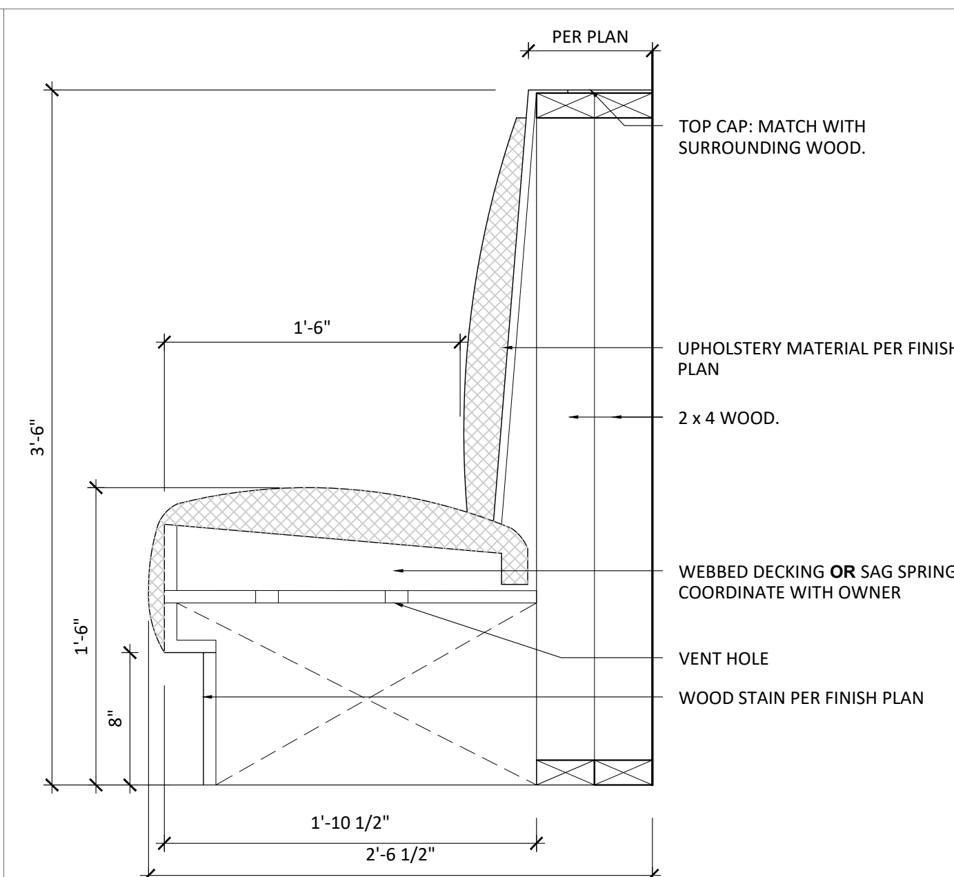
1 BOOTH SEATING SCALE: 1-1/2" = 1'-0"
