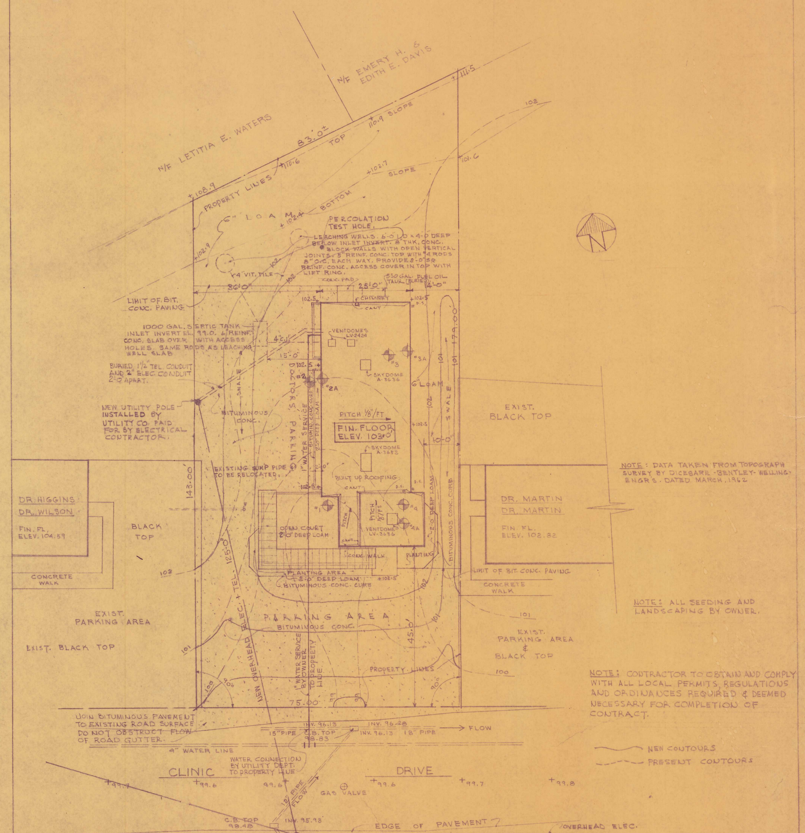
PLOT PLAN SCALE: 1" = 16'
