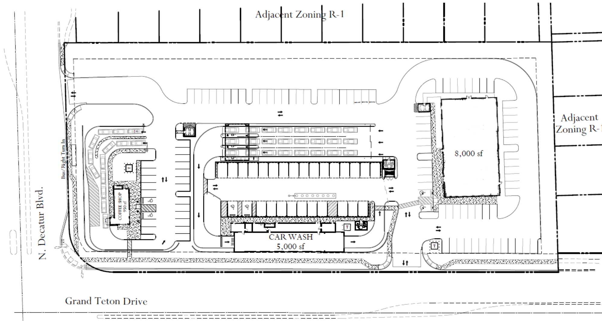
Site Plan with 8,000 sq ft Building
