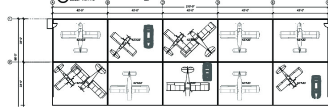
① PRELIMINARY FLOOR PLAN SCALE: 1/8"=1'-0"
