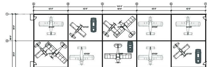
① PRELIMINARY FLOOR PLAN SCALE: 1/8"=1'-0"
