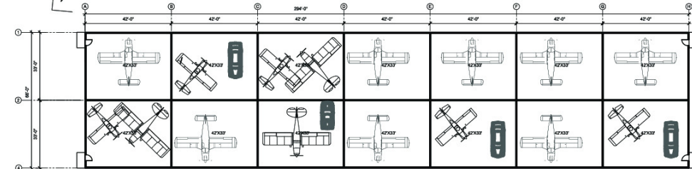
① PRELIMINARY FLOOR PLAN SCALE: 1/8"=1'-0"
