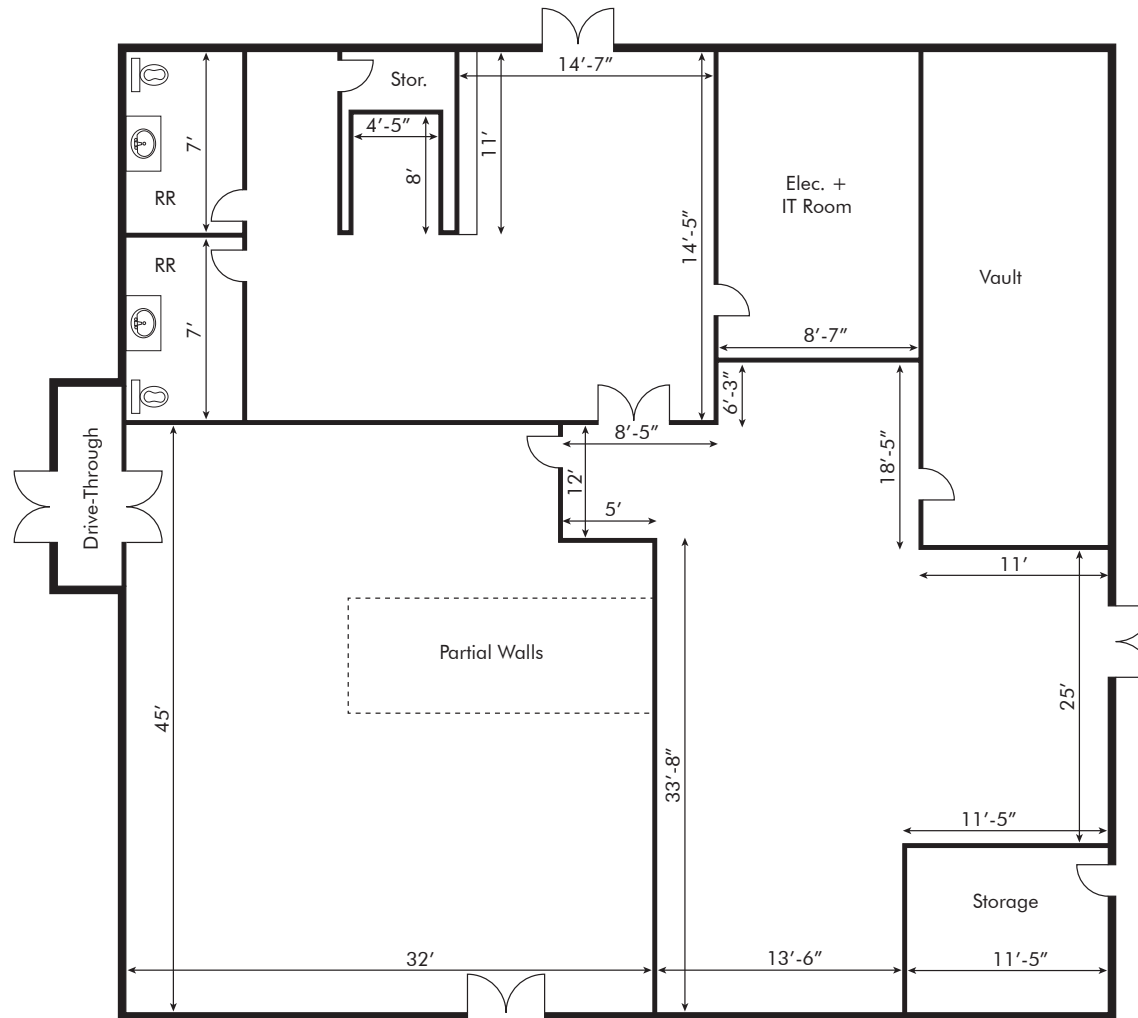
2001 COLUMBUS ST - FLOOR PLAN
