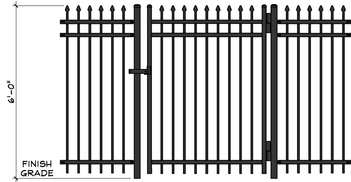
Electric Meter Alcove Security Fence: Ameristar Montage Plus Classic or Equal, Welded Ornamental Steel Fence 4 ft Wide Locking Gate with Lockbox for Power Company Access Color: Black
