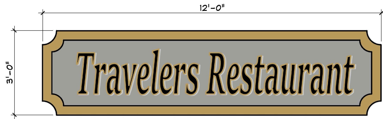
Typical Business Sign Style Mounted to Face of Building Above Storefront Glazing Sign Copy Per Future Commercial Tenants Material: Painted Wood
