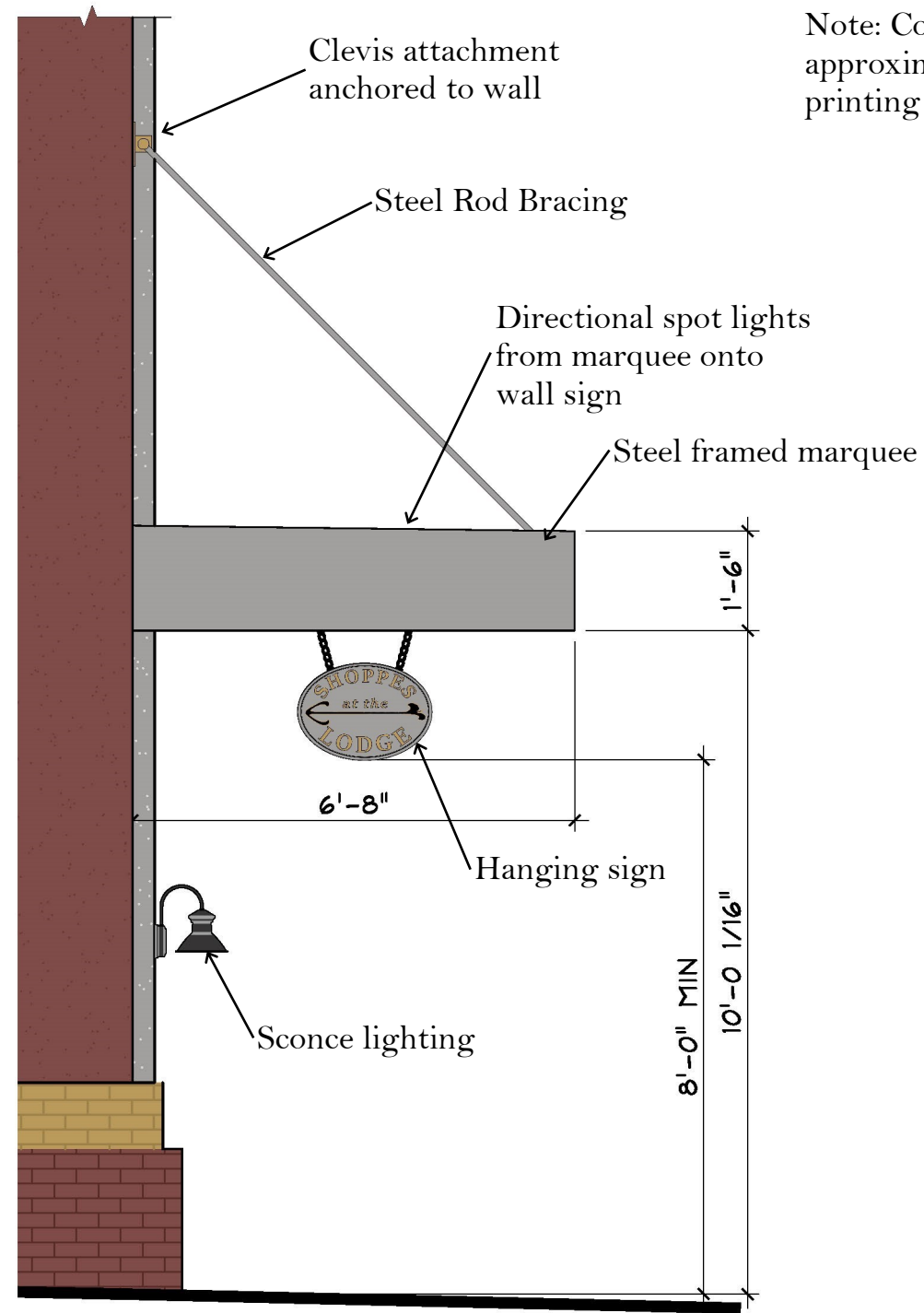
Side Elevation
