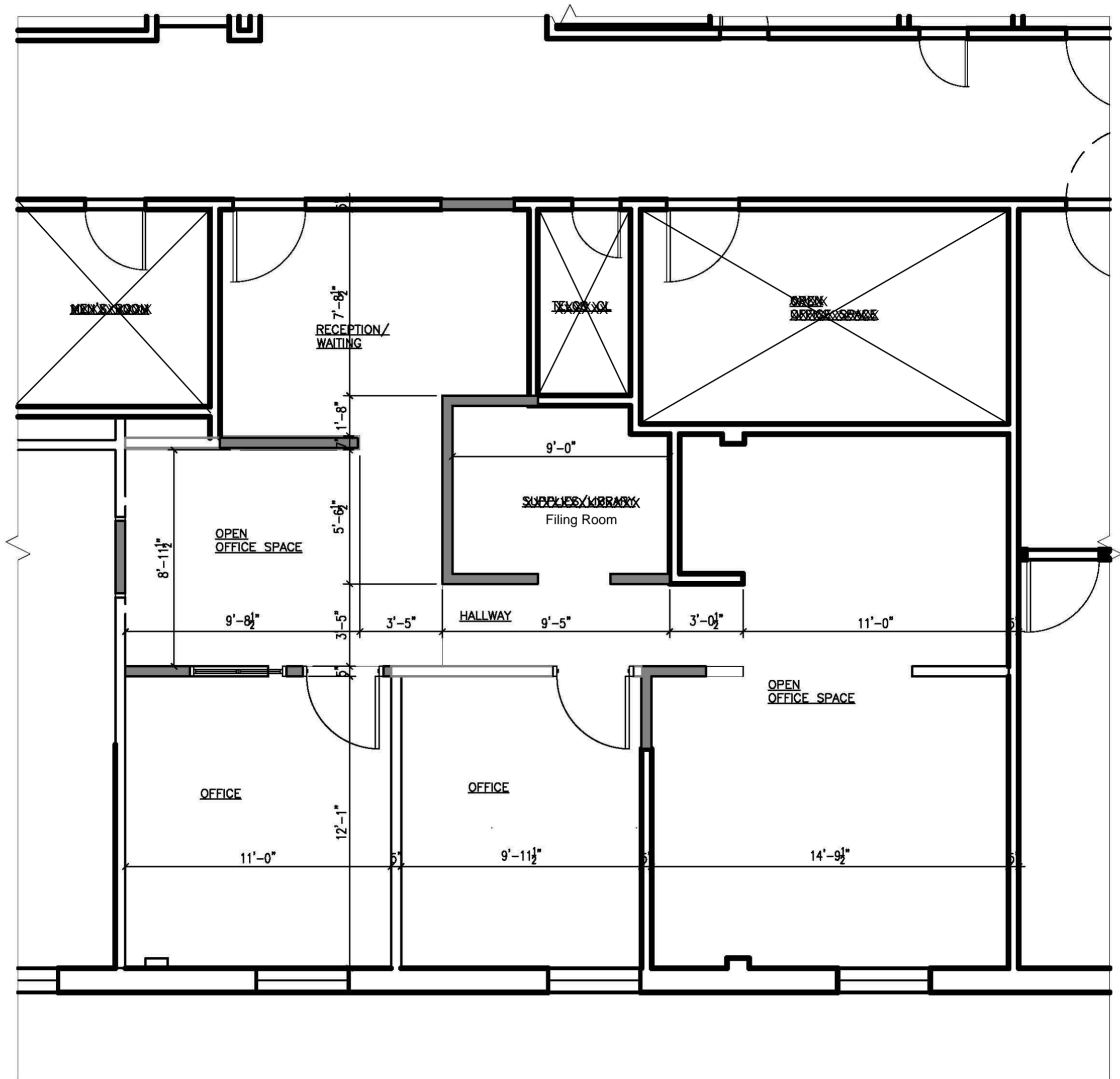
1 SUITES 300 PARTIAL FLOOR PLAN 1/4" = 1'-0"
