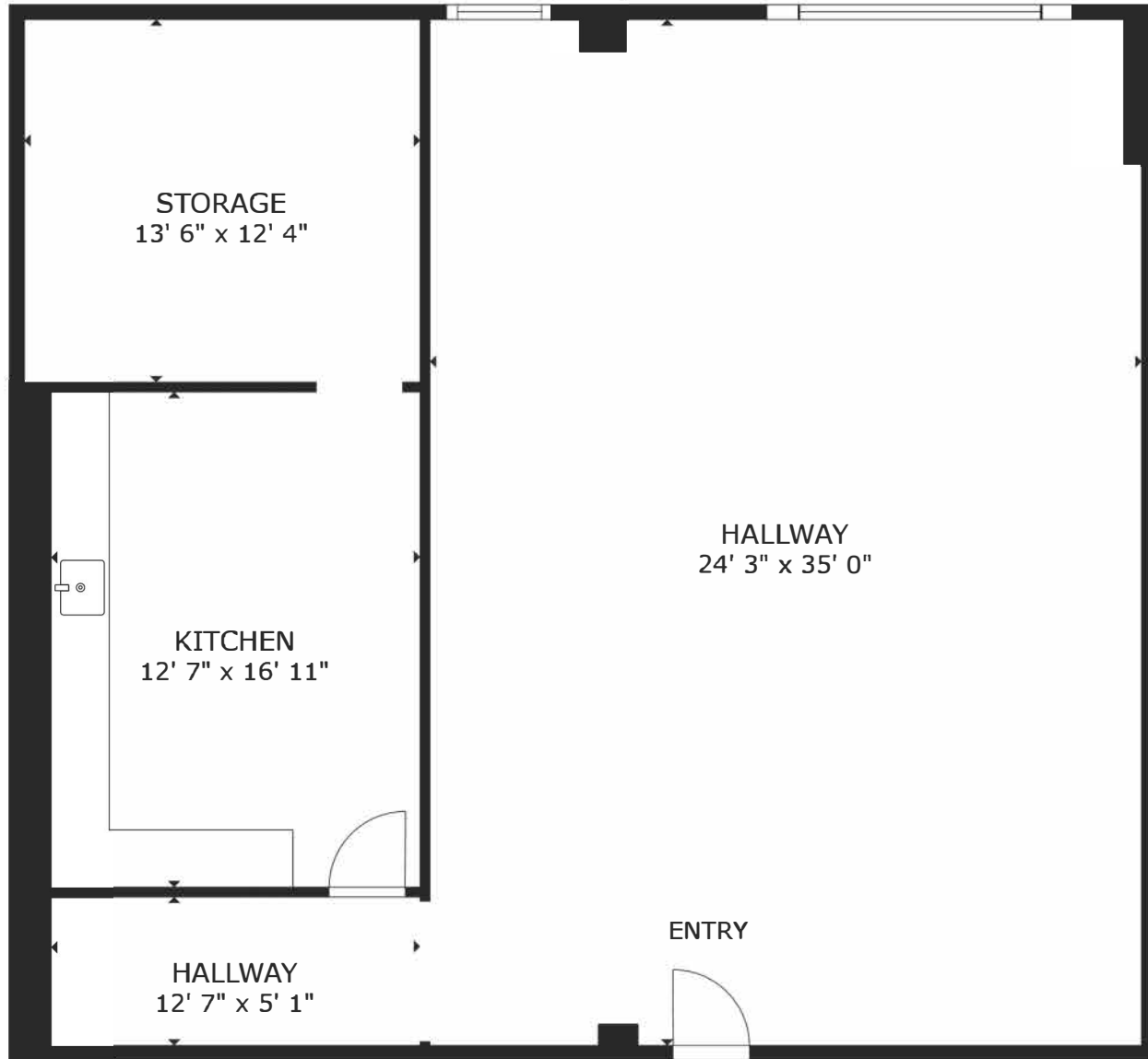
FLOOR PLAN
