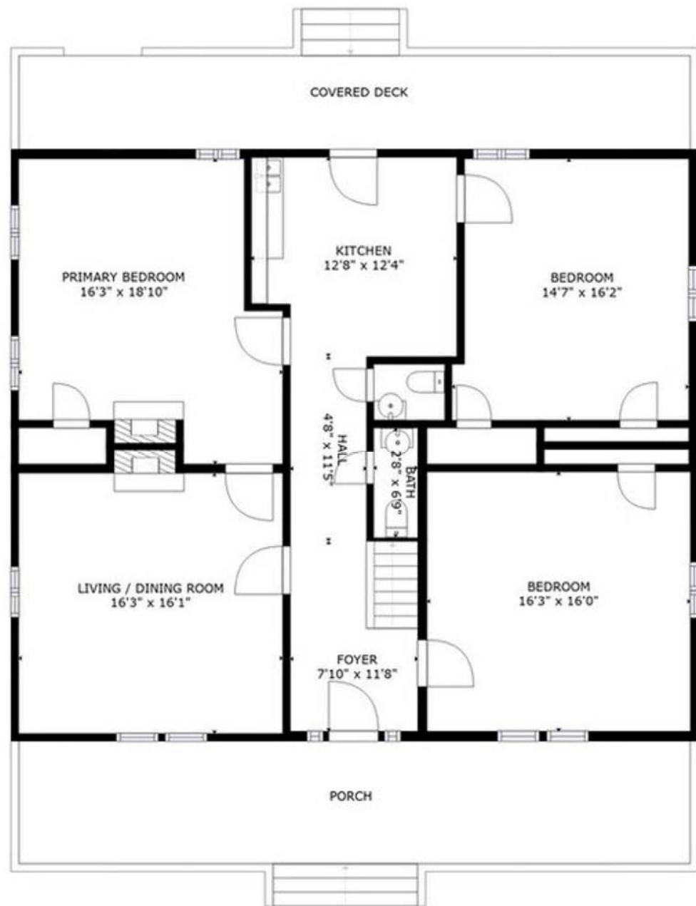
FLOOR 1
