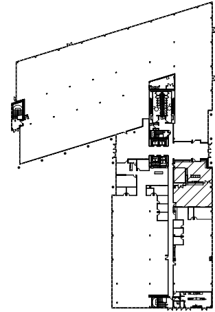
1st Floor Overall Plan
