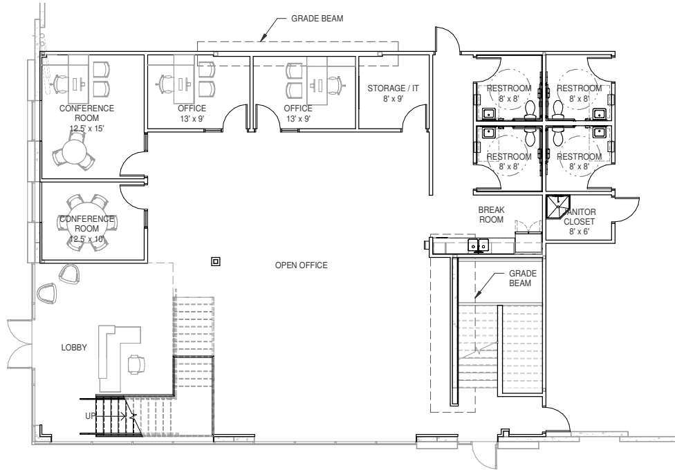
FLOOR 1 ±2,997 SF
