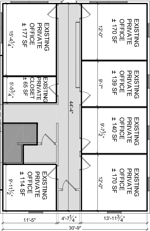
MAIN LEVEL PLAN @ NORTH ADDITION ±1,208 RSF
