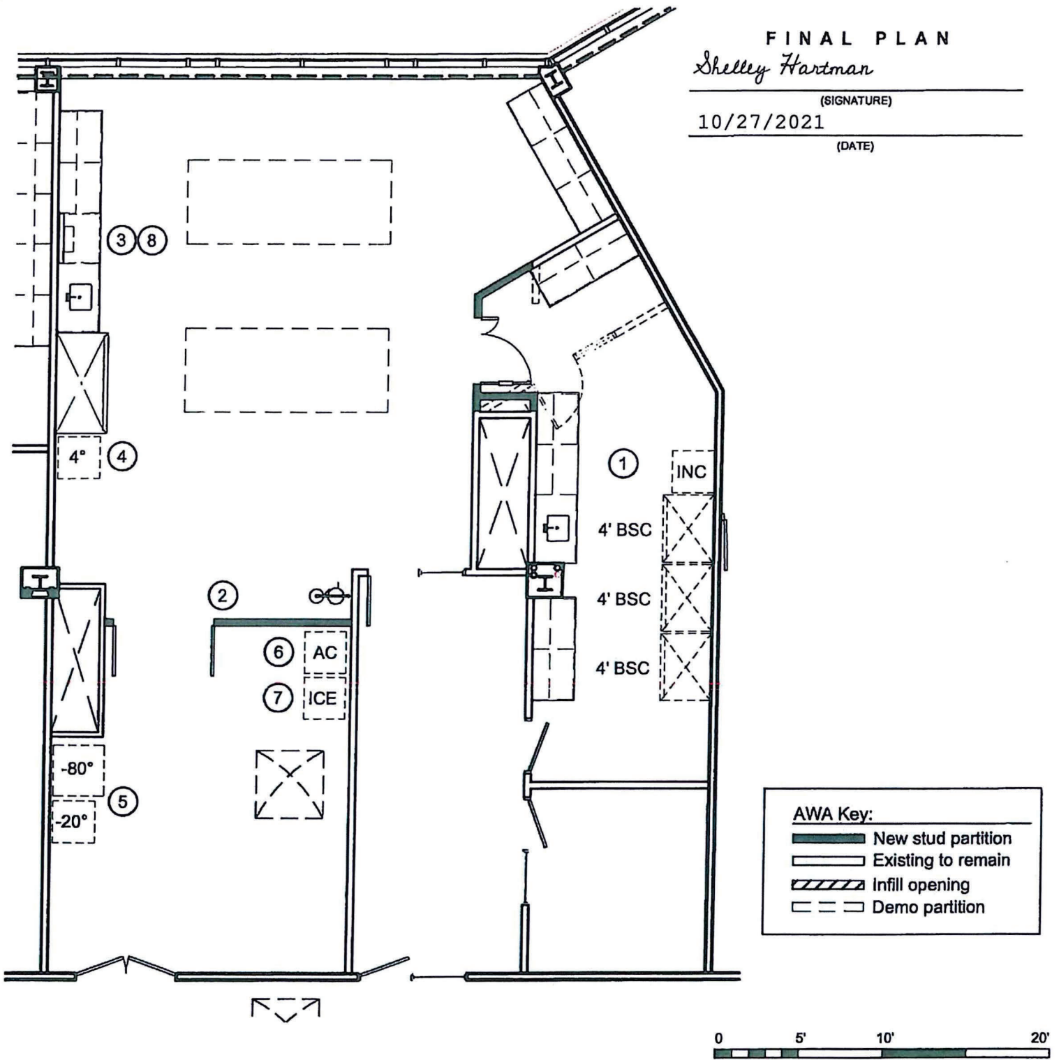
AWA Plan #1
