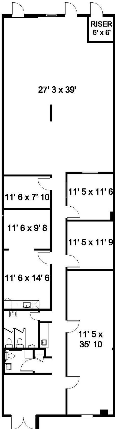
Existing Floor Plan - ±5,850 SF
