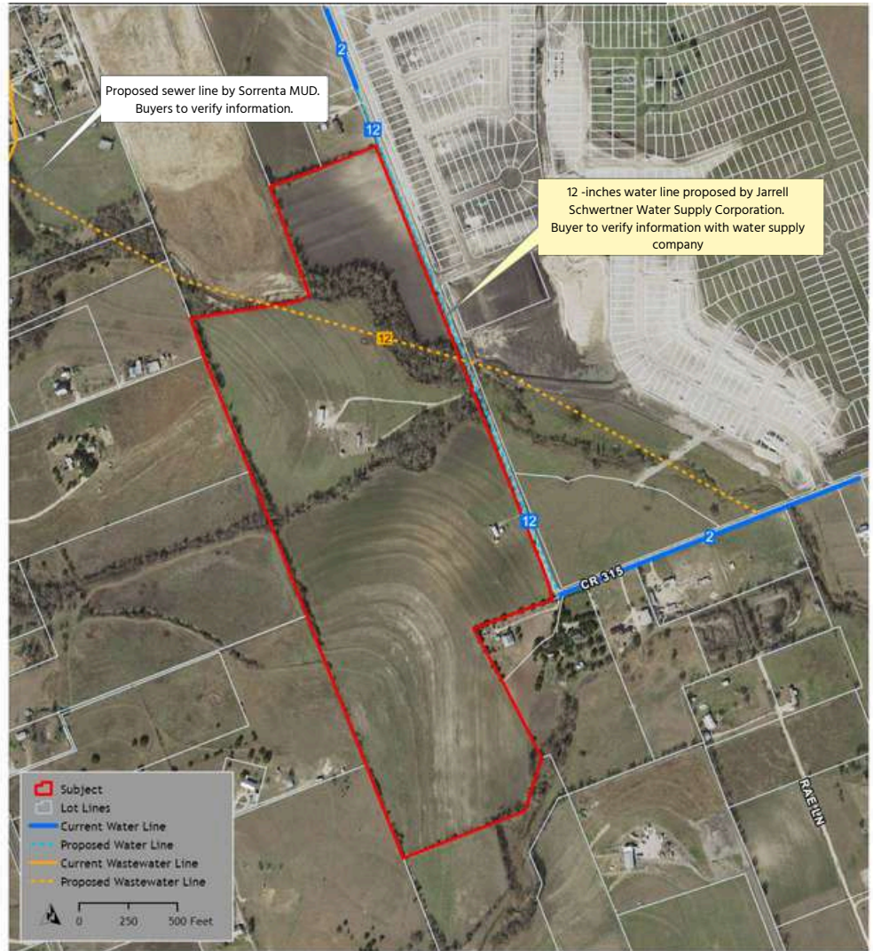
WASTEWATER MAP
