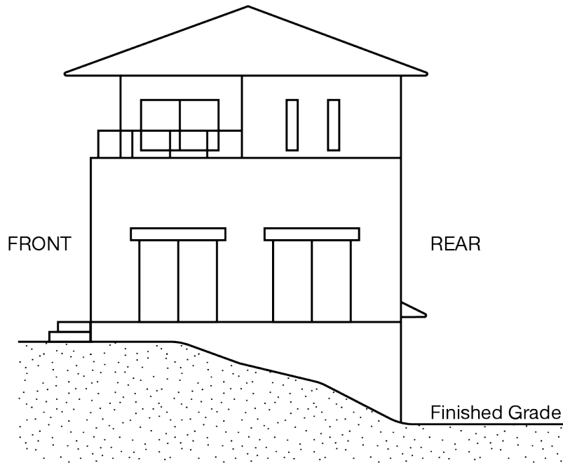
Diagram 2.4 — Walkout Basement
