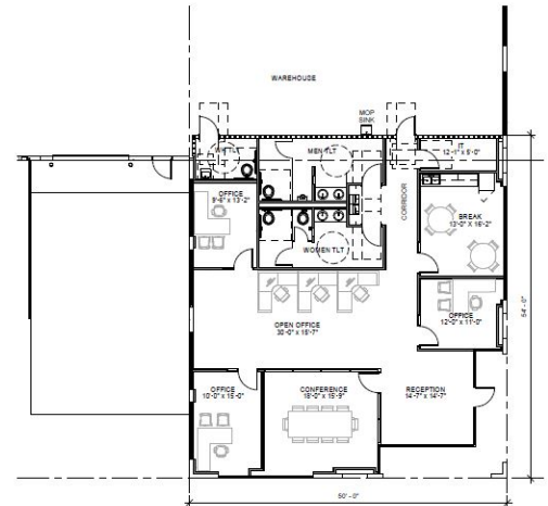
① LEVEL 01 OFFICE SCHEMATIC PLAN 1/8" = 1'-0"
