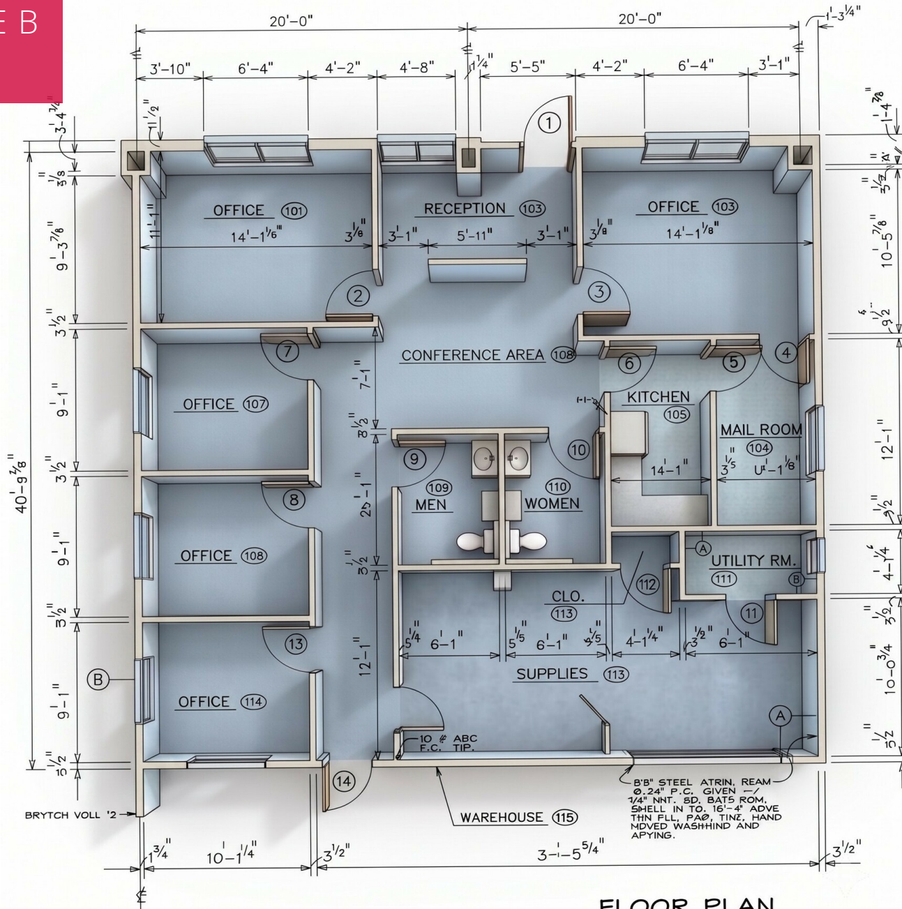
FLOOR PLAN
