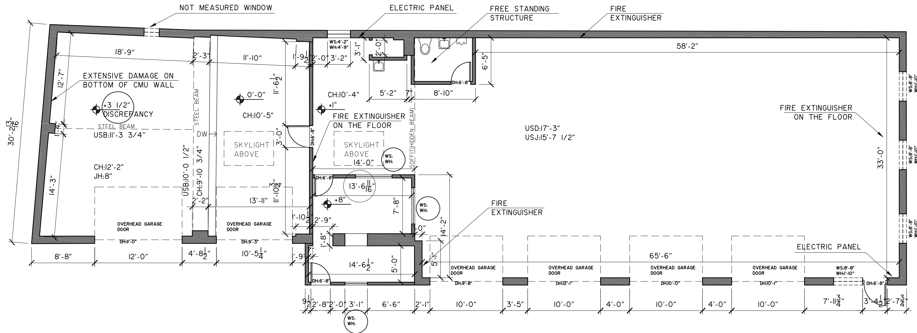
1 EXISTING CONDITIONS PLAN SCALE: 1/8"=1'-0"
