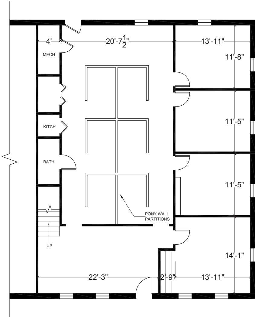
124 MINE LAKE : FIRST FLOOR scale: 1/8"=1'0"
