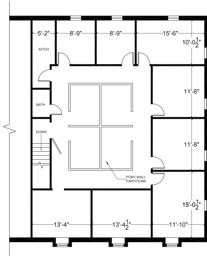
124 MINE LAKE : SECOND FLOOR scale: 1/8"=1'0"
