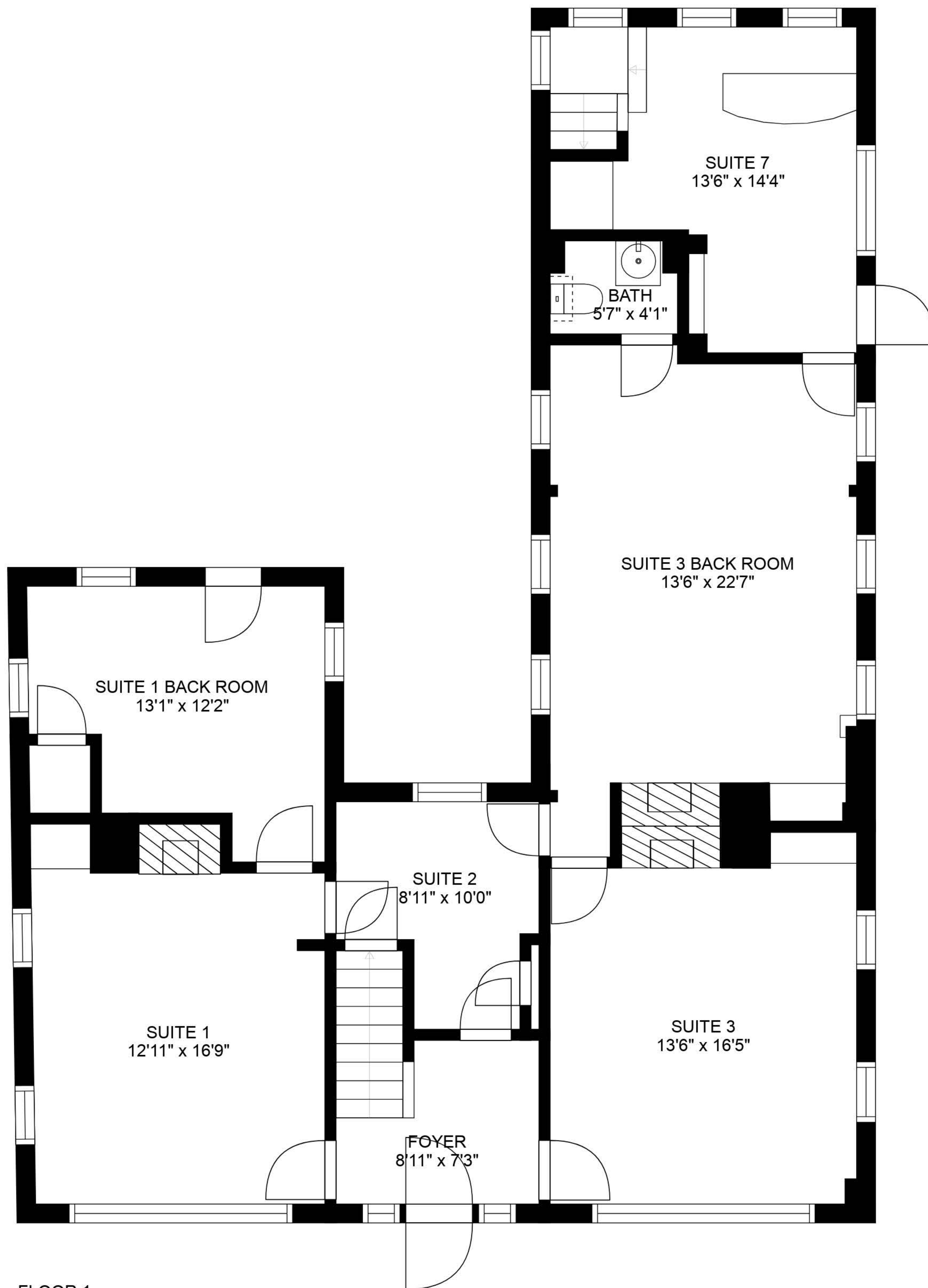
FLOOR 1
