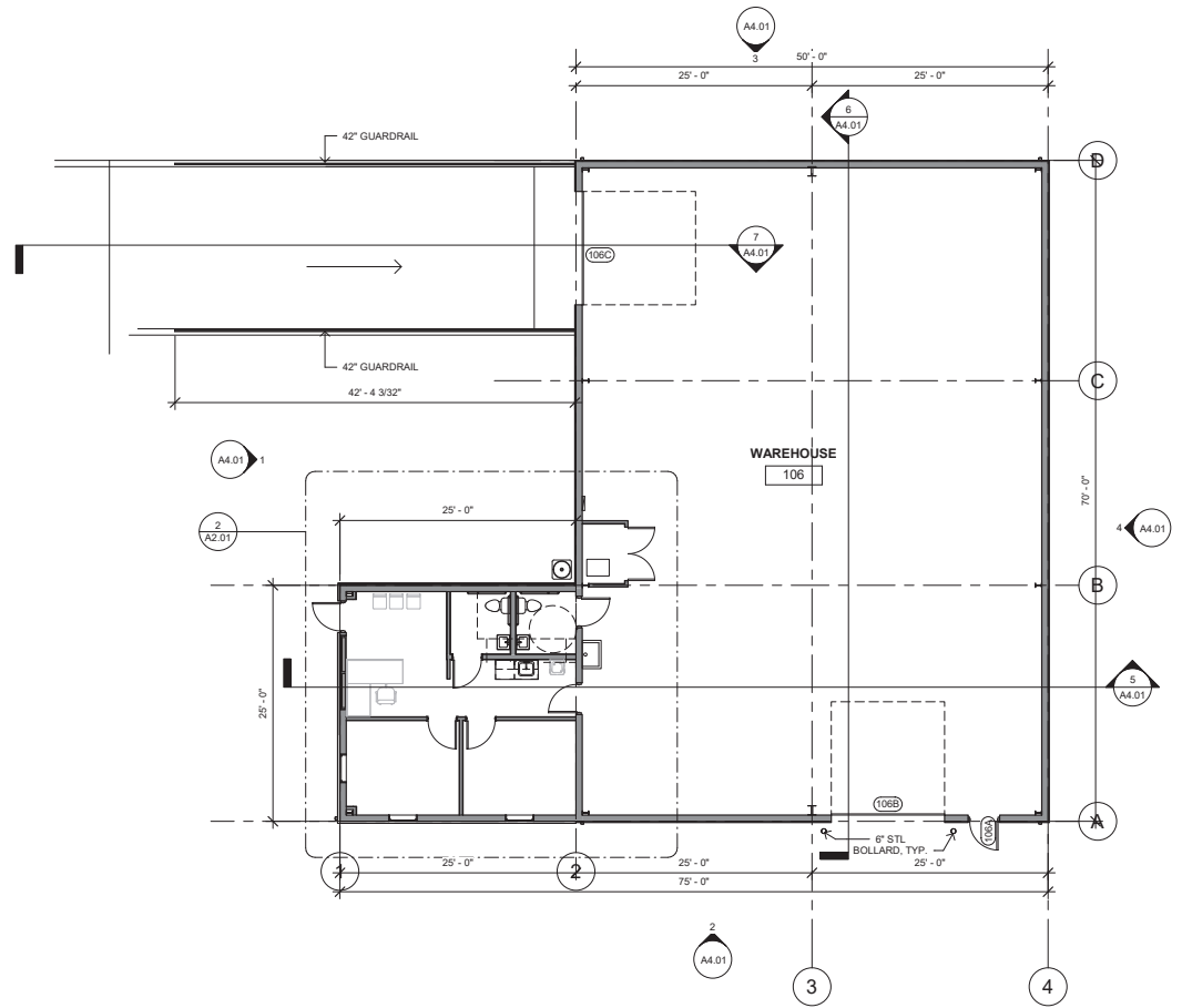
① PROPOSED FLOOR PLAN 1/8" = 1'-0"
