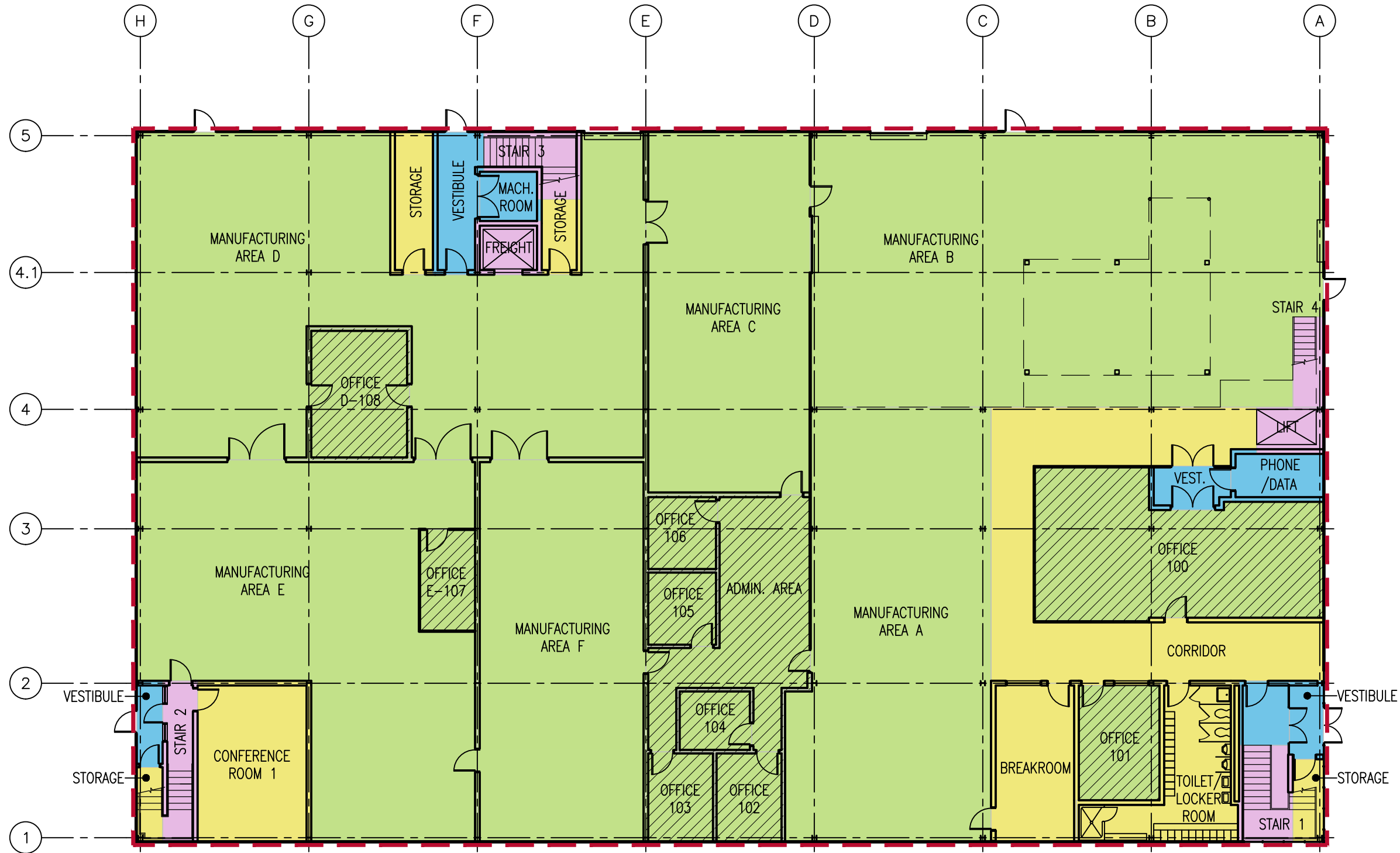
1 FIRST FLOOR PLAN SCALE: 1/16" = 1'-0"
