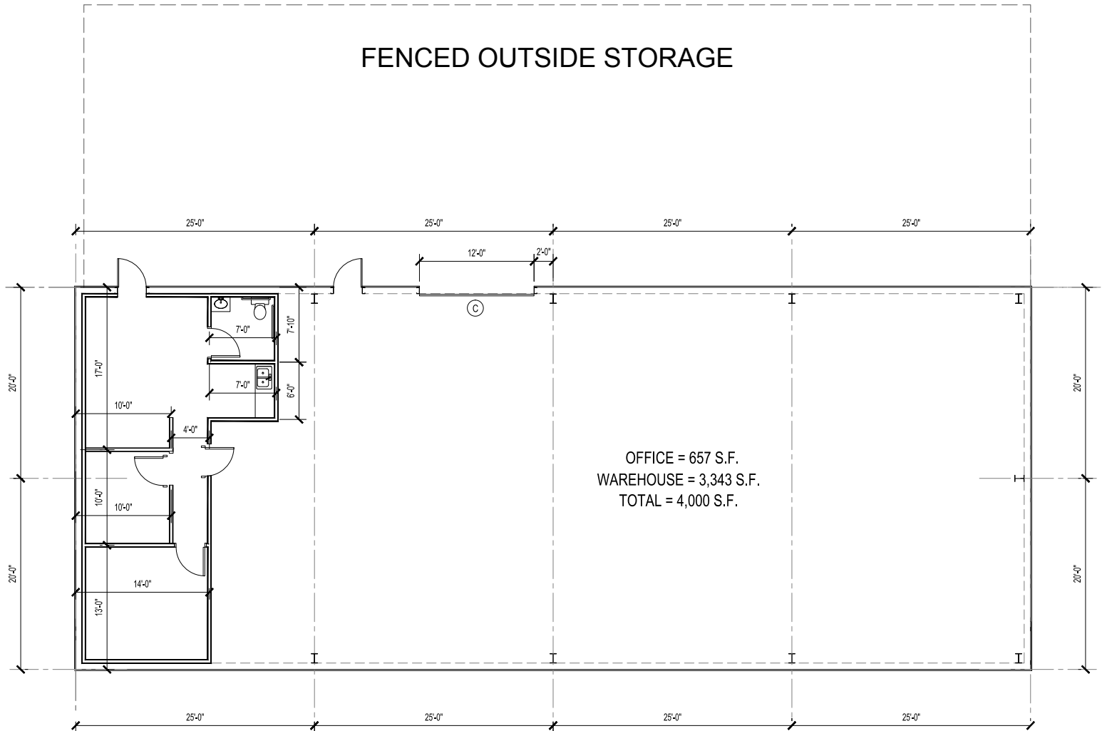
FLOOR PLAN 3/16"=1'-0"
