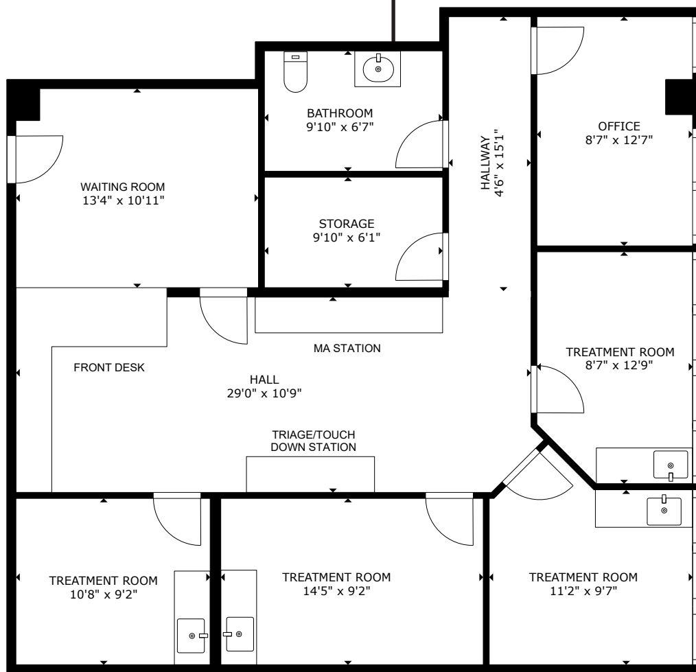
FLOOR PLAN
