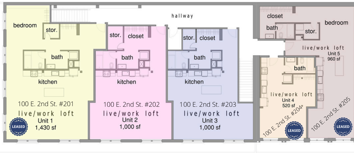
2nd & main lofts second floor plan
