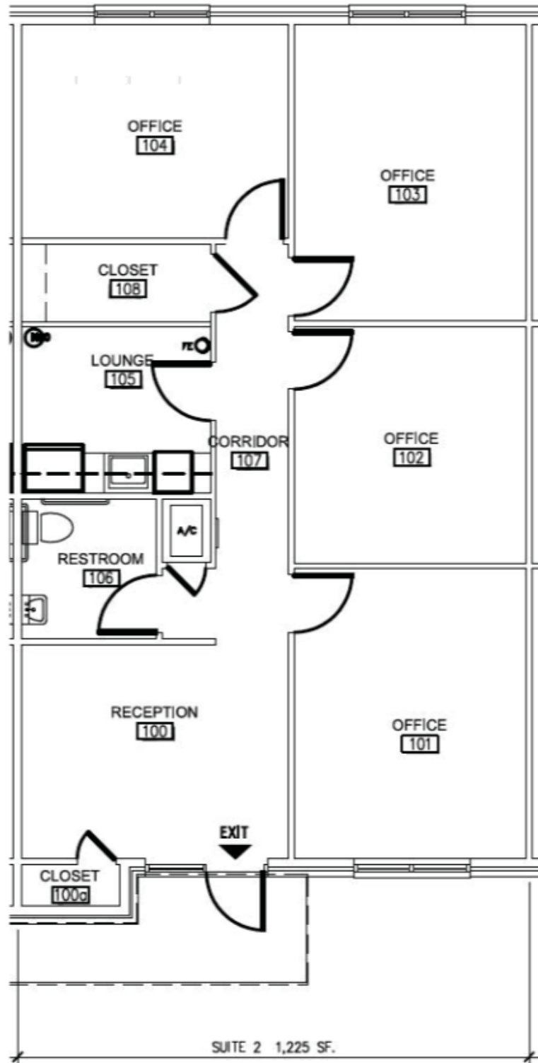
FLOOR PLAN - MIDDLE UNIT 1,225 SQFT
