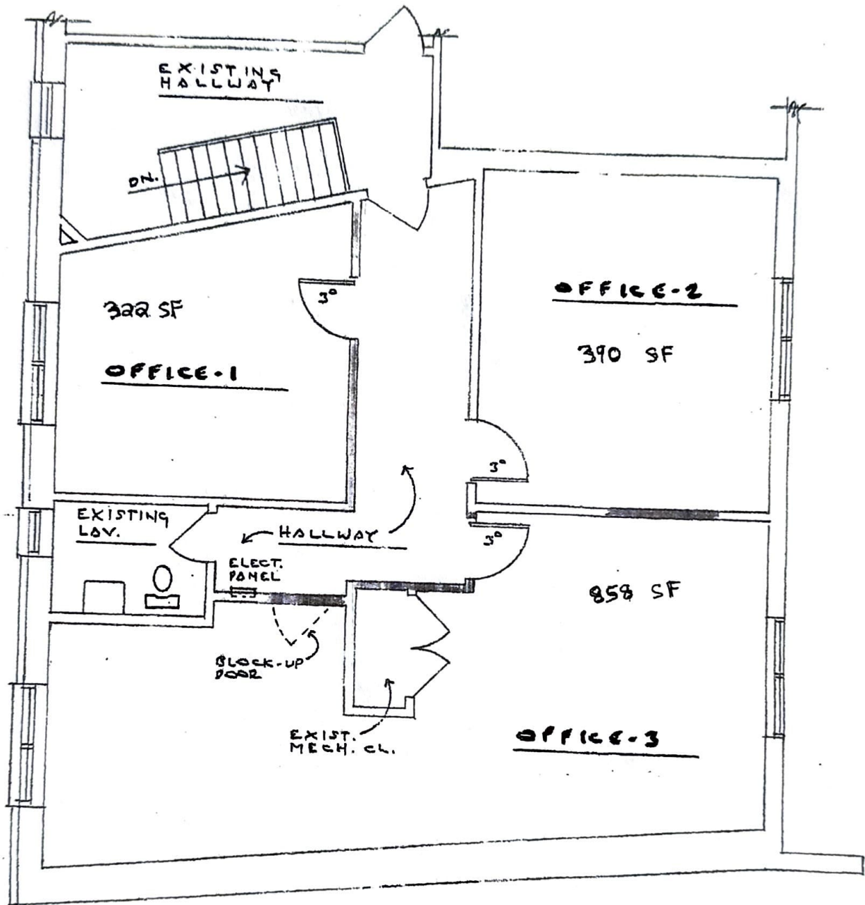
SECOND FLOOR PLAN SUITE - 2A (3 NEW OFFICES)
