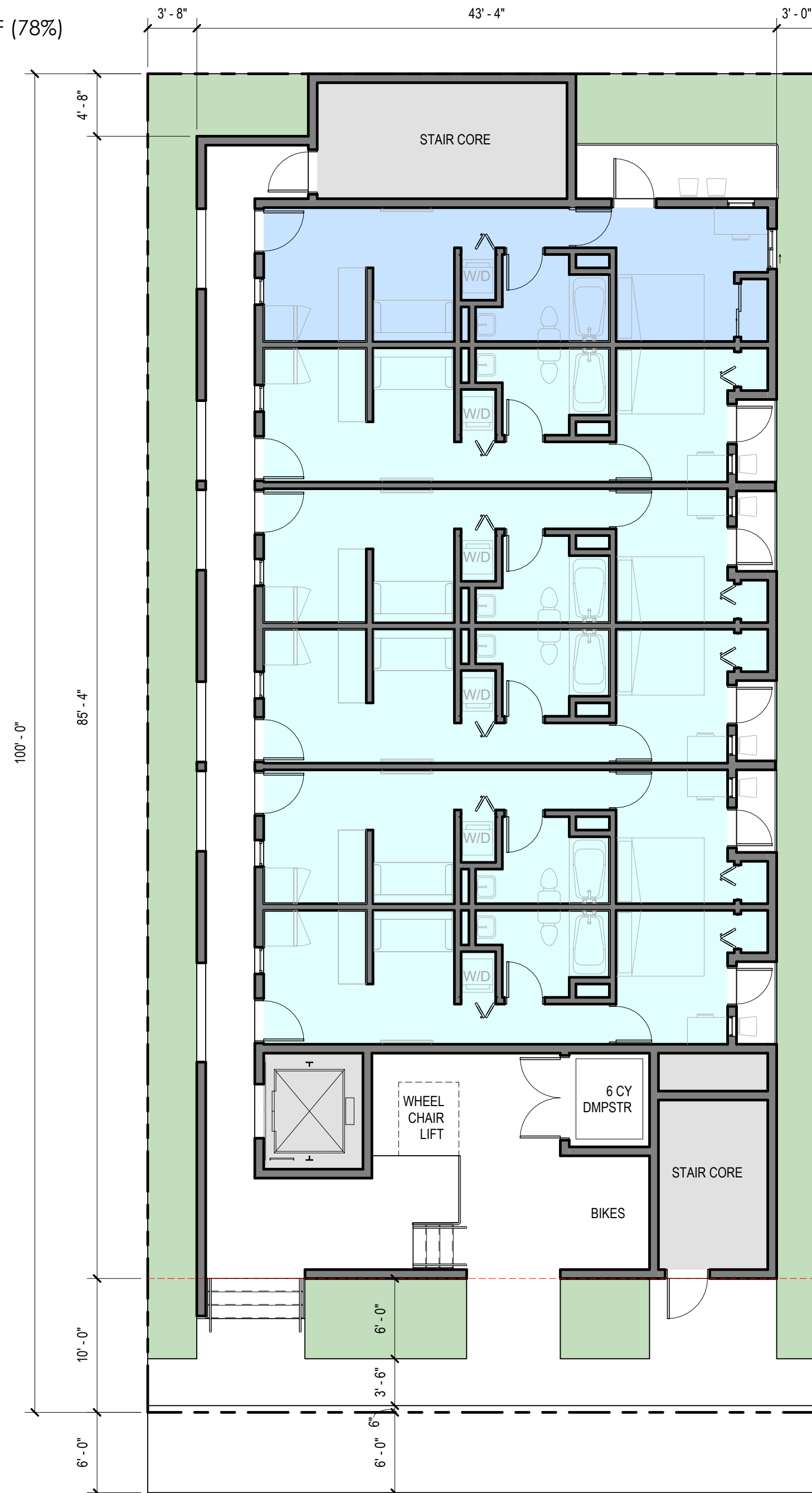
1 LEVEL 1 1/8" = 1'-0"
