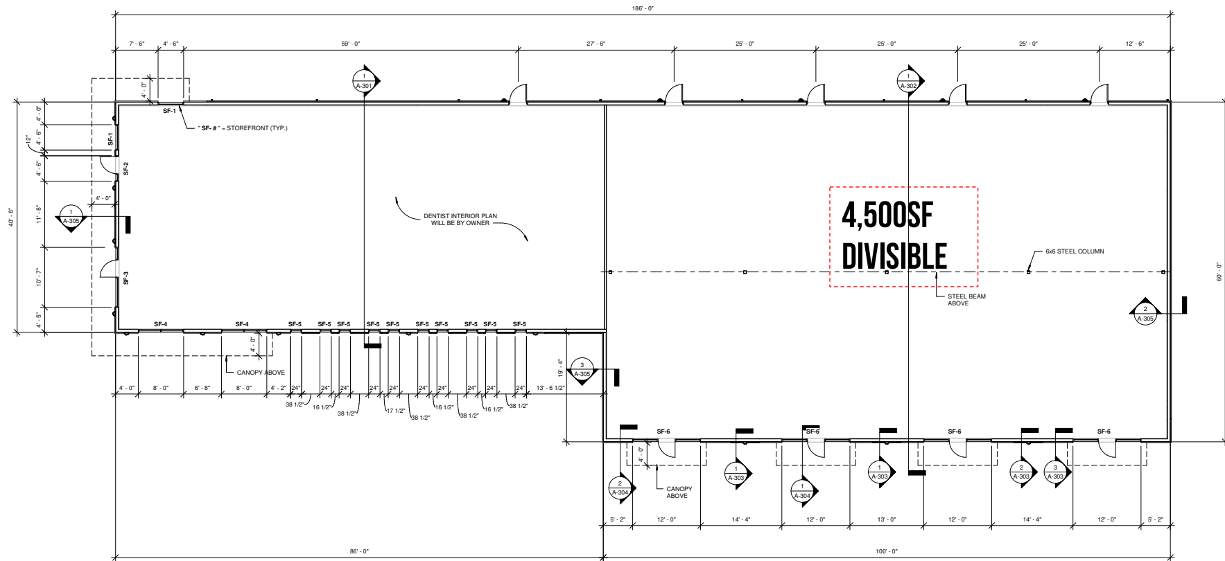
① FLOOR PLAN 1/8" = 1'-0"
