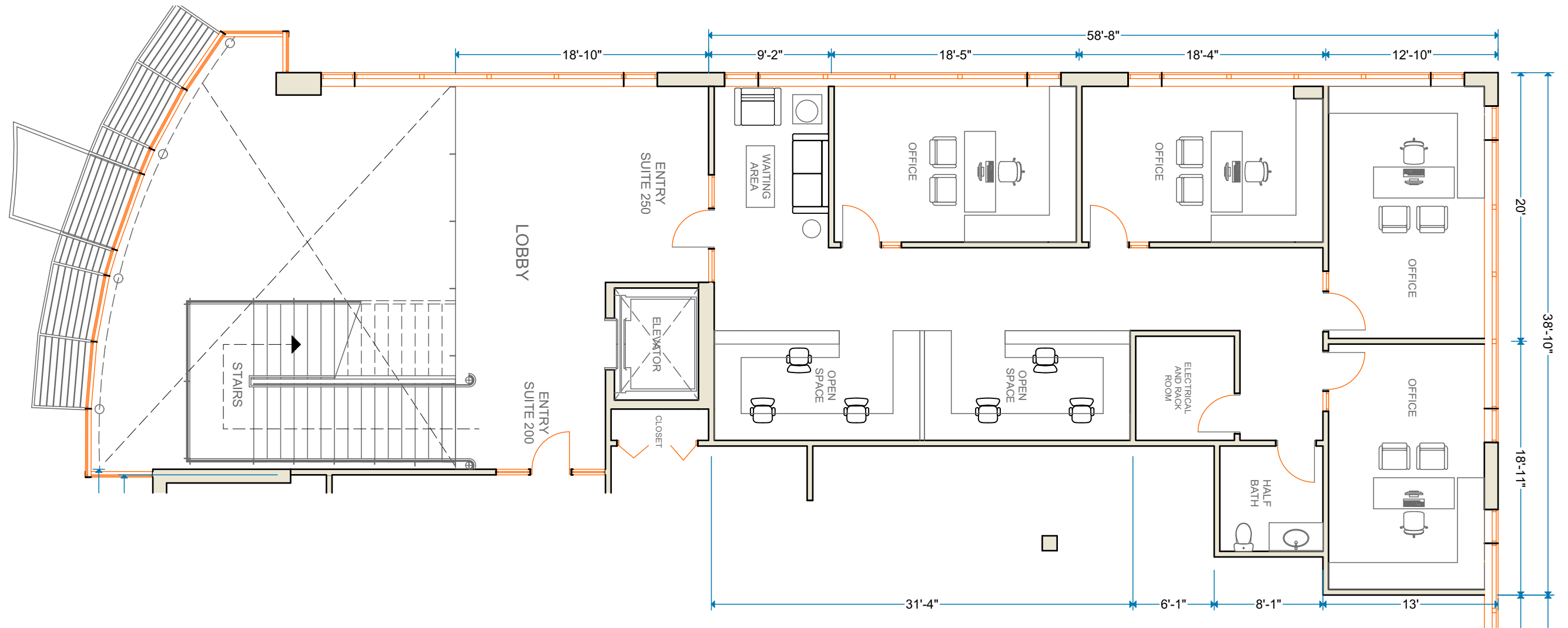
FLOOR PLAN
