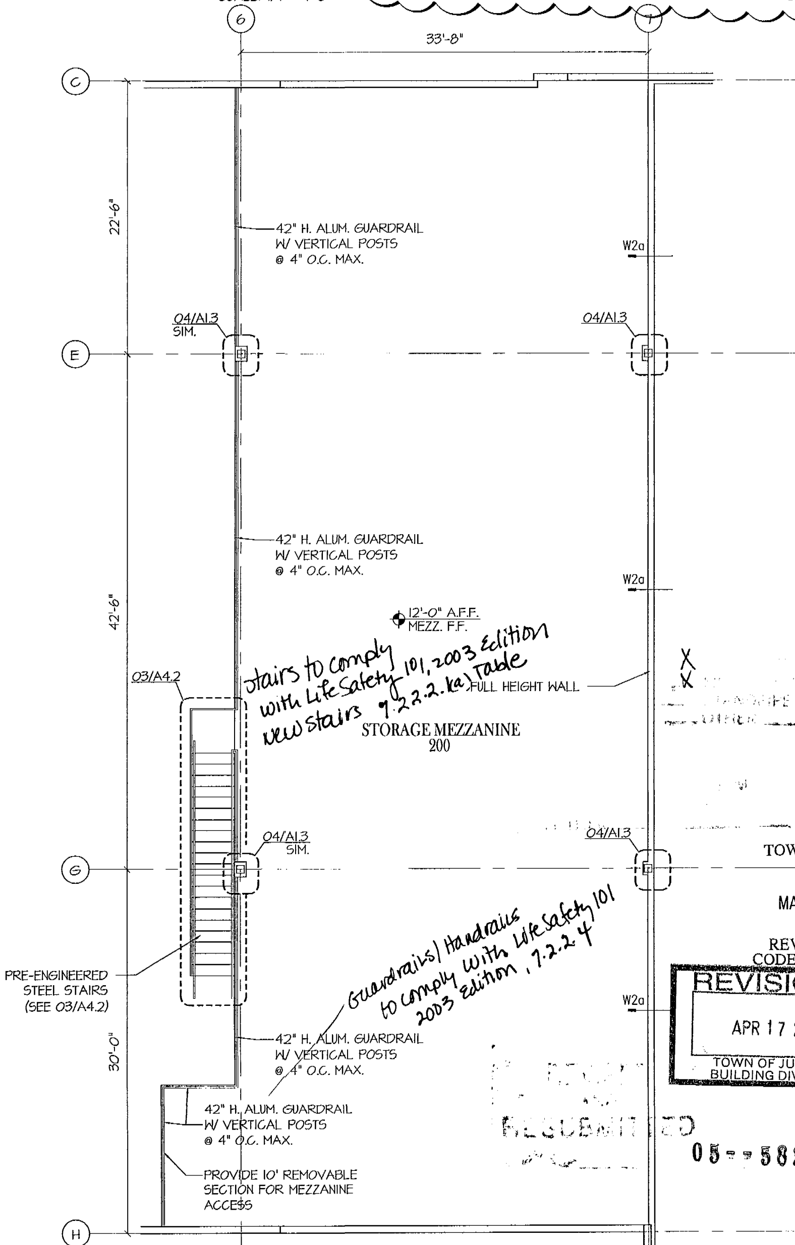
MEZZANINE PLAN
