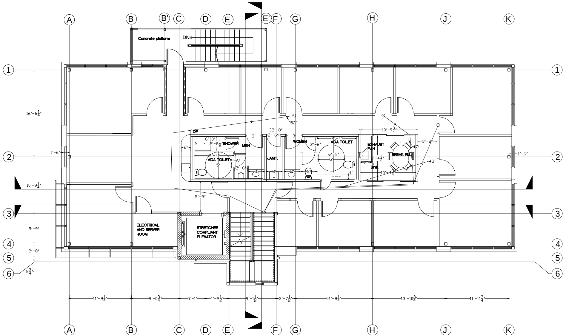
4TH FLOOR Scale: 1/4"=0"
