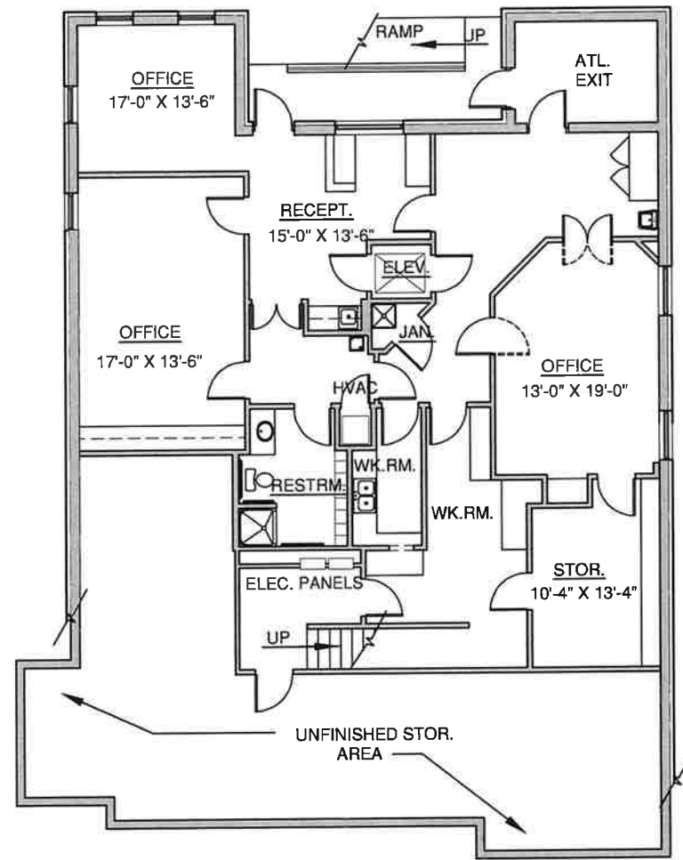
BASEMENT LEVEL FLOOR PLAN EXISTING CONDITIONS - TOTAL NET SQ. FT. = 2061
