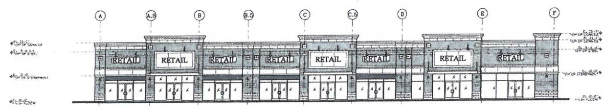
02 FRONT ELEVATION SCALE 1/8" = 1'-0"
