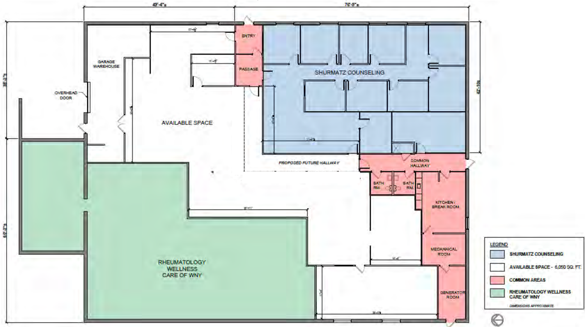
Floor Plan
