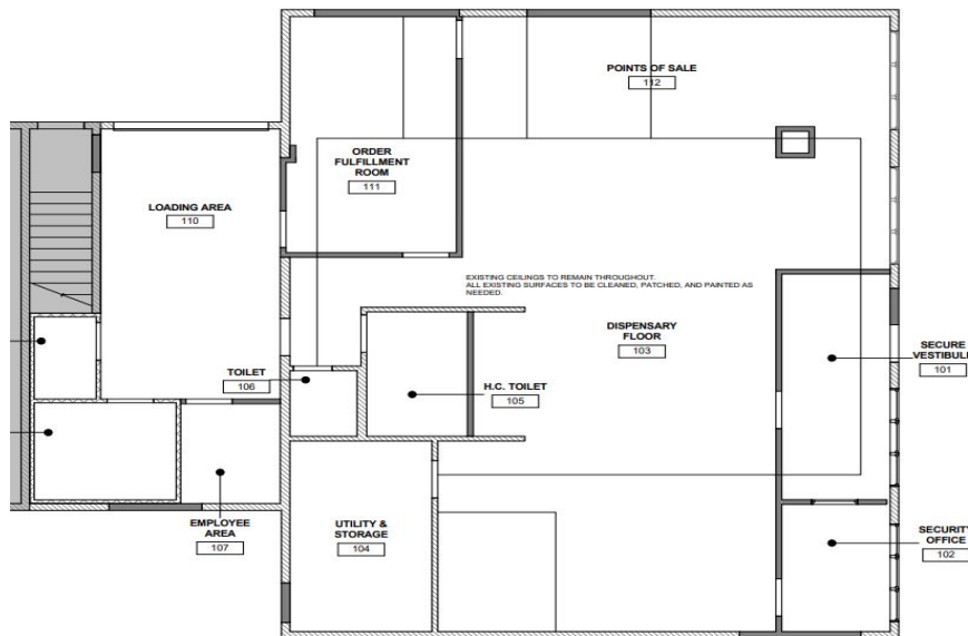
① MAIN LEVEL REFLECTED CEILING PLAN 1/4" = 1'-0"
