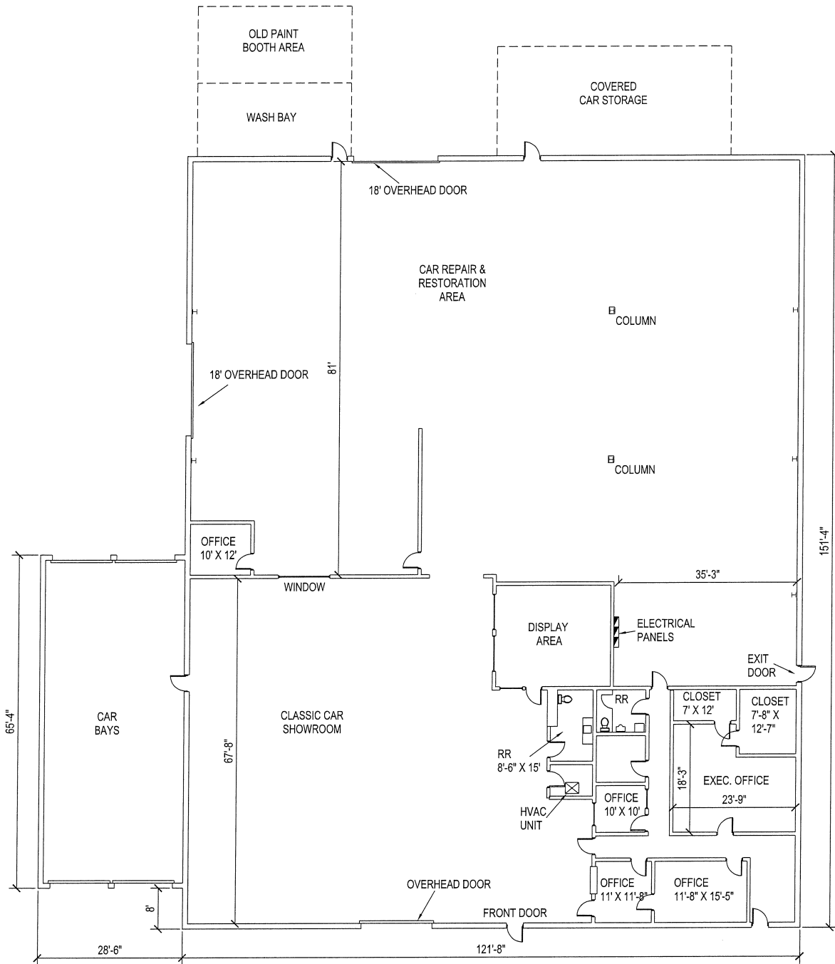
FLOOR PLAN - 20,274 SQ. FT. 7200 HARRY HINES BLVD. DALLAS, TEXAS
