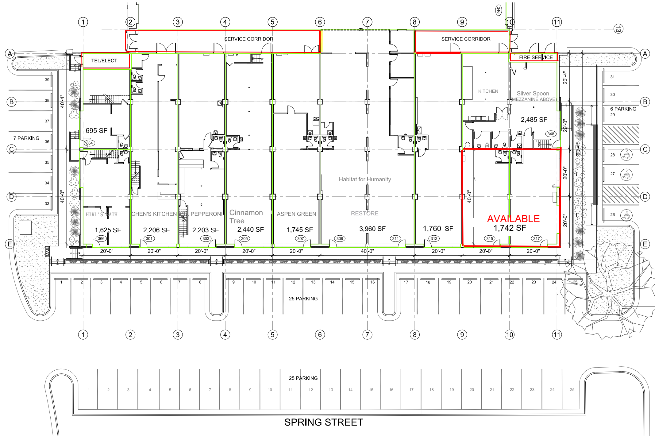
1 RESTON HERNDON BUSINESS PARK - BUILDING 3A MAIN FLOOR 3A-1 NOT TO SCALE
