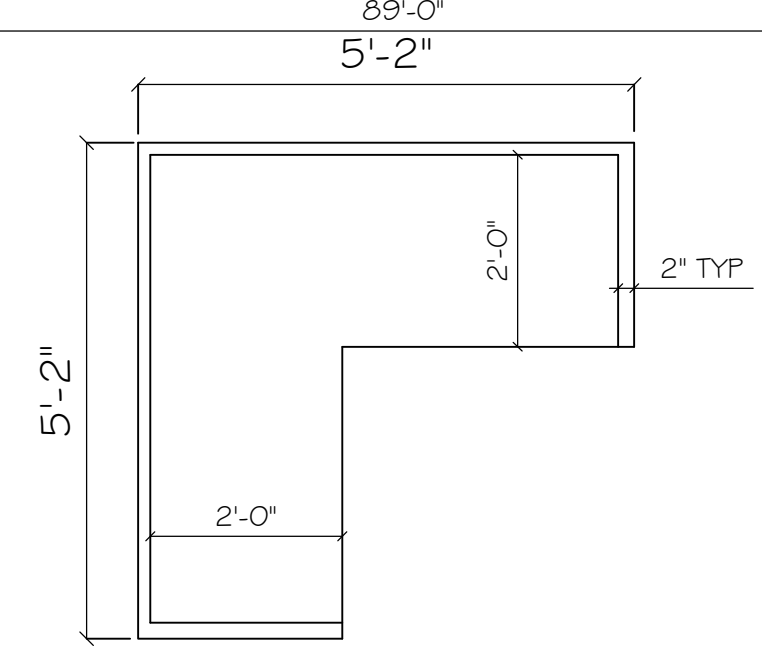
TYPICAL CUBE IS DRAWN TO ABOVE DIMENSIONS WITH 1" SHOWN BETWEEN ALL CUBES—SCALE 1/2" = 1'-0"
