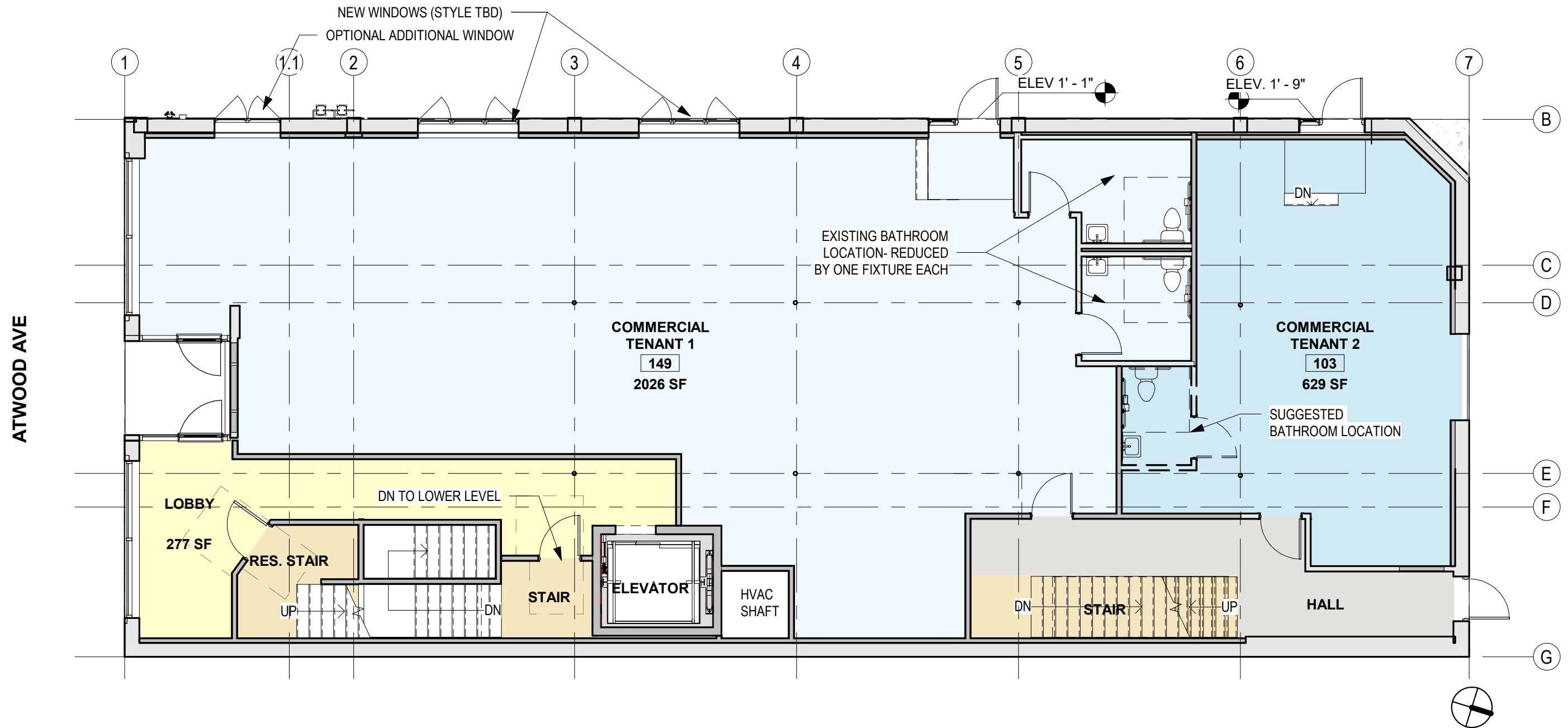
1- FLR Phase 1 Concept 11x17 1/8" = 1'-0"
